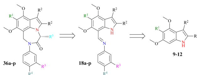
Scheme 1 Retrosynthesis of designed indole-based diazepines 36a–p .
