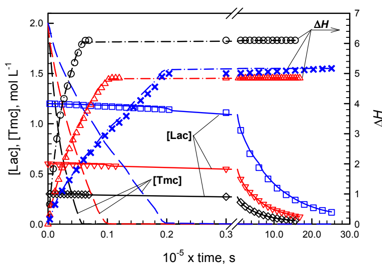
Figure 2. Experimental and simulated evolution of [Lac] , [Tmc] , and \Delta H in copolymerizations initiated with R - Ini for different [Lac]_0 : 0.3 (black), 0.6 (red), and 1.2 mol·L -1 (blue). Experimental data marked by symbols, simulated data by lines. Other initial conditions: [Tmc]_0 = 2 mol·L -1 . [R\text{-Ini}]_0 = 2 \times 10^{-3} mol·L -1 ( + [{}^iPrOH]_0 = 4 \times 10^{-3} mol·L -1 due to in situ synthesis of Ini ).
