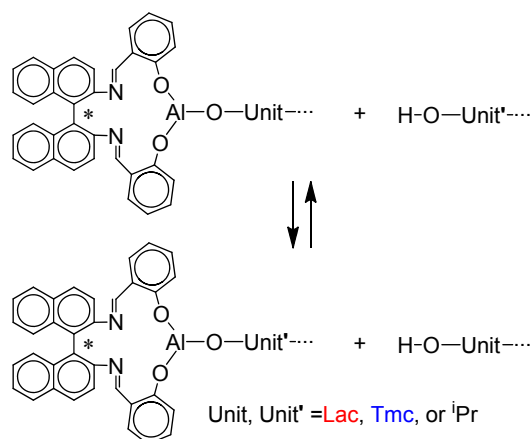
Scheme 6. Chain-transfer reactions operating in the studied copolymerization systems. Due to the assumption of instantaneous initiation isopropyl ( i Pr) containing active species, as well as i PrOH, coming from the in situ synthesis of Ini (cf. Scheme 3), could be neglected.
