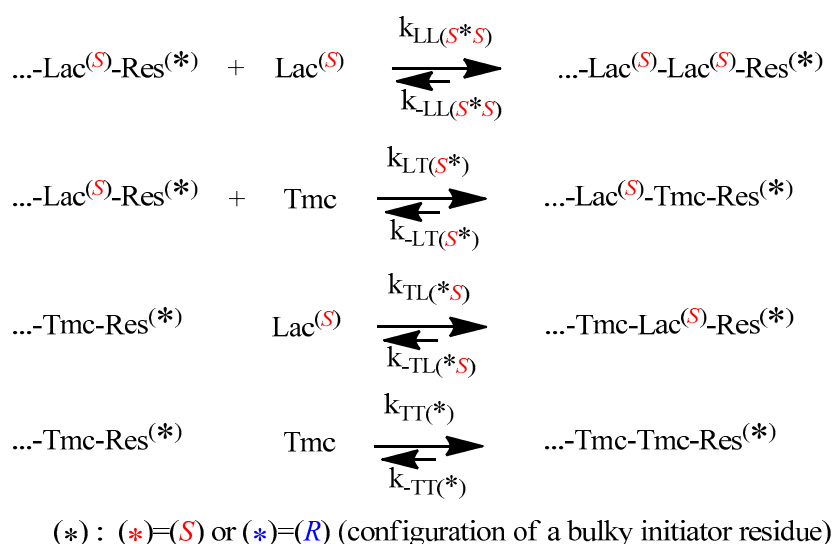
Scheme 4. Chemical reactions governing copolymerization of Lac with Tmc . ‘Res’ denotes the asymmetric residue coming from initiator.
