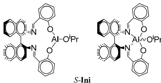
Scheme 2. Structure of S -2,2'-[1,1'-binaphthyl-2,2'-diyl-bis-(nitrylomidylidene)]-diphenoxy aluminum isopropoxide ( S - Ini ). R - Ini enantiomer differs with conformation of binaphthyl residue, restricted due to inhibited rotation. Although the pentacoordinated structure is probably dominating in the reaction medium, we, for the sake of simplification, use tricoordinated structures in our other schemes.
