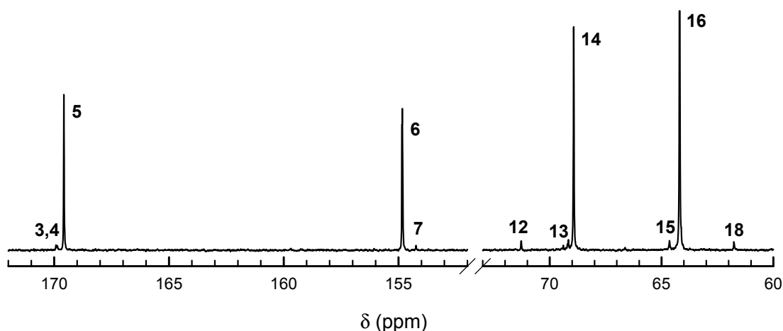
Figure 4. ^{13}\text{C} NMR spectra of Tmc/Lac copolymers prepared with R -Ini. Polymerization conditions: [\text{Lac}]_0 , [\text{Tmc}]_0 , [\text{R-Ini}]_0 = 1.2 , 2 , and 2 \times 10^{-3} ( [\text{iPrOH}]_0 = 4 \times 10^{-3} ) \text{mol}\cdot\text{L}^{-1} , respectively. Time 3.81 \times 10^6 s, conversion Lac = 92%, conversion Tmc = 99%. Note large contributions of signals of homo Lac and Tmc sequences, signals 13, and 15, respectively. Assignment of signals is given in Table 1.
