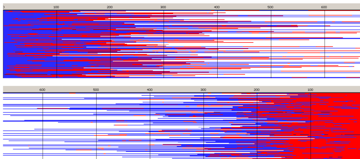
Figure 6. Sample of simulated chains in copolymerization initiated with Tmc-R-Ini * . Reactivity ratios as given in Table 2, z_{LL} = 3.8 \times 10^{-3} , k_{ex}/k_{TT} = 4 \times 10^{-2} . [Tmc]_0 = 2 , [Lac]_0 = 1.2 \text{ mol}\cdot\text{L}^{-1} , and [Ini]_0 = 2 \times 10^{-3} \text{ mol}\cdot\text{L}^{-1} ( [iPrOH]_0 = 4 \times 10^{-3} \text{ mol}\cdot\text{L}^{-1} due to in situ synthesis of Ini ). Conversion 95%, DP_n = 507.4 , D = 1.48 , average number of homoblocks per chain equal to 5.2. Red and blue mark Lac and Tmc units, respectively. Top box: unit positions numerated starting from chain beginning; bottom box: starting units numeration from chain-end. For the sake of plots clarity the chains longer than DP = 1.3 DP_n are shown only partially (this applies also to similar plots below).
