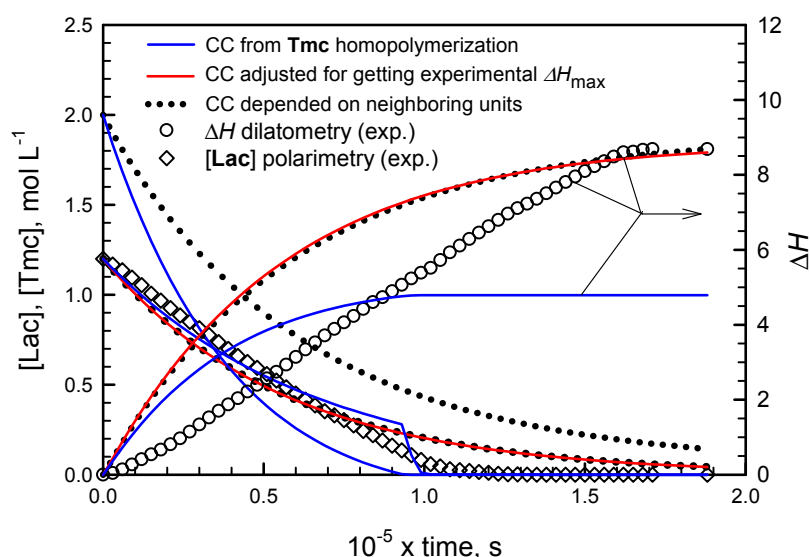
Figure 1. Fitting of simulated changes of [Lac] (lines starting from [Lac] = 1.2) and of the dilatometer meniscus height \Delta H (lines starting from \Delta H = 0 ) to experimental data (diamonds: [Lac] , circles: meniscus \Delta H ) for copolymerization of Lac with Tmc , initiated with [S\text{-Ini}] = 2 \times 10^{-3} ( +[\text{iPrOH}]_0 = 4 \times 10^{-3} mol·L -1 due to in situ synthesis of Ini ), [\text{Lac}]_0 = 1.2 , [\text{Tmc}]_0 = 2 mol·L -1 . Blue lines: volume contraction coefficient (CC) for Tmc copolymerization equal to that determined from homopolymerization experiments, red lines: CC for Tmc units increased to get the same final meniscus height as determined experimentally, black dot lines: Tmc and Lac unit CC depending on neighboring units, as determined in our studies (see Supporting Information). Additionally the predicted changes of [Tmc] are presented (lines starting from [Tmc] = 2).
