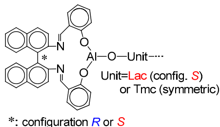
Scheme 5. Schematic presentation of the active chain-end in copolymerization of Lac with Tmc .
