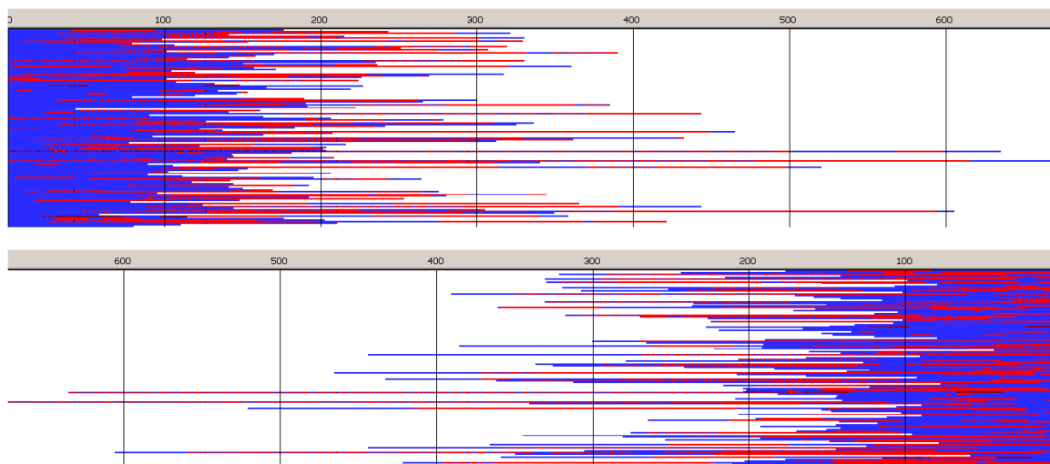
Figure 10. Sets of simulated copolymer chains in copolymerization initiated with the mixture of R - and S - Ini (94:6). Reactivity ratios as given in Table 2, z_{LLR} = 6.92 , z_{LLS} = 1.45 , and the ratio of Tmc homopropagation rate constants, k_{TTR}/k_{TTS} , being about 0.78. [\text{Tmc}]_0 = 2 , [\text{Lac}]_0 = 1.2 \text{ mol}\cdot\text{L}^{-1} , and [\text{Ini}]_0 = 5 \times 10^{-3} ( +[^i\text{PrOH}]_0 = 1 \times 10^{-2} , due to in situ synthesis of Ini ), Conversion 95%, DP_n = 202.1 , \bar{D} = 1.27 , average number of homoblocks in a chain equal to 25.2.
