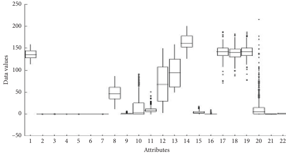
FIGURE 4: Boxplot of CTG attributes.
