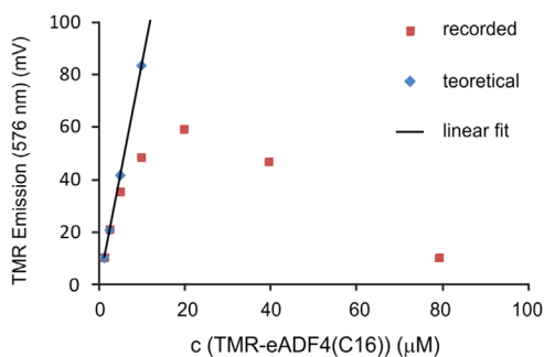
Fig. 2. Emission intensity of tetramethylrhodamine fluorescence plotted against concentration of labeled TMR-eADF4(C16) (red squares) in comparison to the theoretical linear intensity of the dye based on the emission of labeled protein at the lowest concentration (1.2 \mu\text{M} ) (blue diamonds) reveal a strong inner filter effect of the tetramethylrhodamine label.
