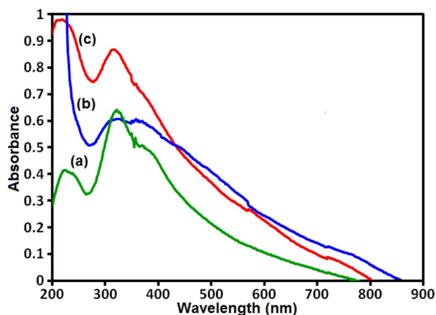
Fig. 7 UV-vis DRS spectra of (a) g\text{-C}_3\text{N}_4 , (b) \text{CoFe}_2\text{O}_4 and (c) g\text{-C}_3\text{N}_4/\text{CoFe}_2\text{O}_4 nanocomposite.
