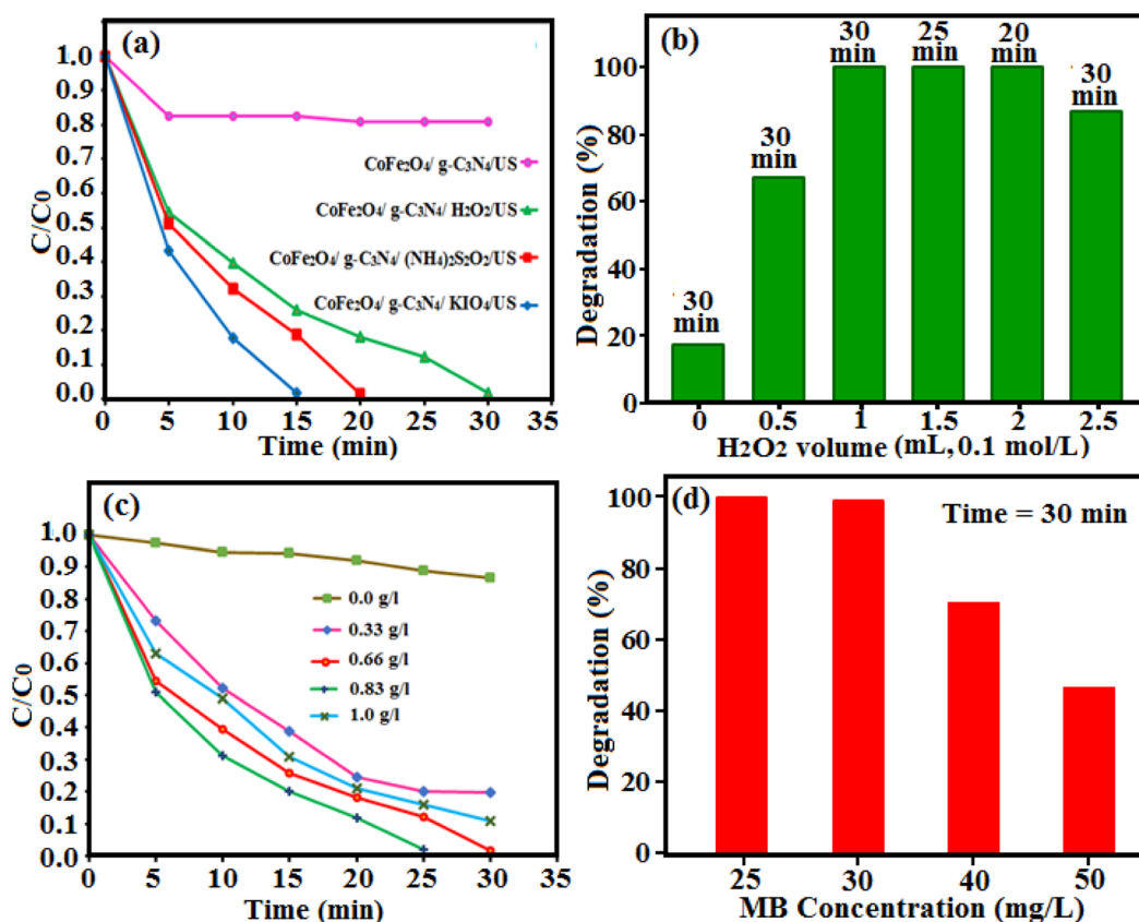
Fig. 11 Effects of (a) different enhancers, (b) the \text{H}_2\text{O}_2 amount, (c) the g\text{-C}_3\text{N}_4/\text{CoFe}_2\text{O}_4 sonocatalyst dosage, and (d) initial dye concentration on the sonocatalytic degradation of MB in the presence of g\text{-C}_3\text{N}_4/\text{CoFe}_2\text{O}_4 nanocomposite. Conditions: [\text{MB}]_0 = 25 \text{ mg L}^{-1} , 50 mL; [enhancer] = 0.1 \text{ mol L}^{-1} , 1 mL; [cat.] = 0.66 \text{ g L}^{-1} at room temperature and natural pH = 7.
