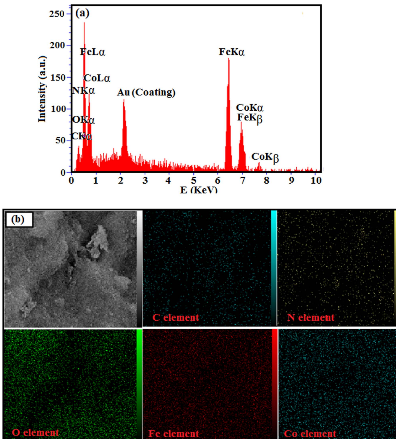
Fig. 4 (a) The EDX spectrum and (b) elemental mappings of g\text{-C}_3\text{N}_4/\text{CoFe}_2\text{O}_4 nanocomposite.
