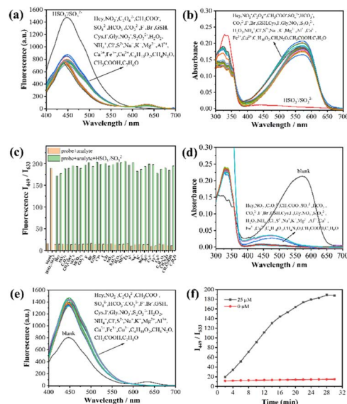
Fig. 2 (a) The fluorescence emission spectra of TLA (5 μM) responding to various analytes. (b) The absorption spectra of TLA (5 μM) responding to various analytes. (c) The I 449 /I 633 value of TLA (5 μM) toward HSO 3 - /SO 3 2- in the presence of other analytes. (d) The absorption spectra of TLA (5 μM) toward HSO 3 - /SO 3 2- in the presence of other analytes. (e) The fluorescence emission spectra of TLA (5 μM) toward HSO 3 - /SO 3 2- in the presence of other analytes. (f) The responding time of TLA (5 μM) toward HSO 3 - /SO 3 2- (25 μM).
