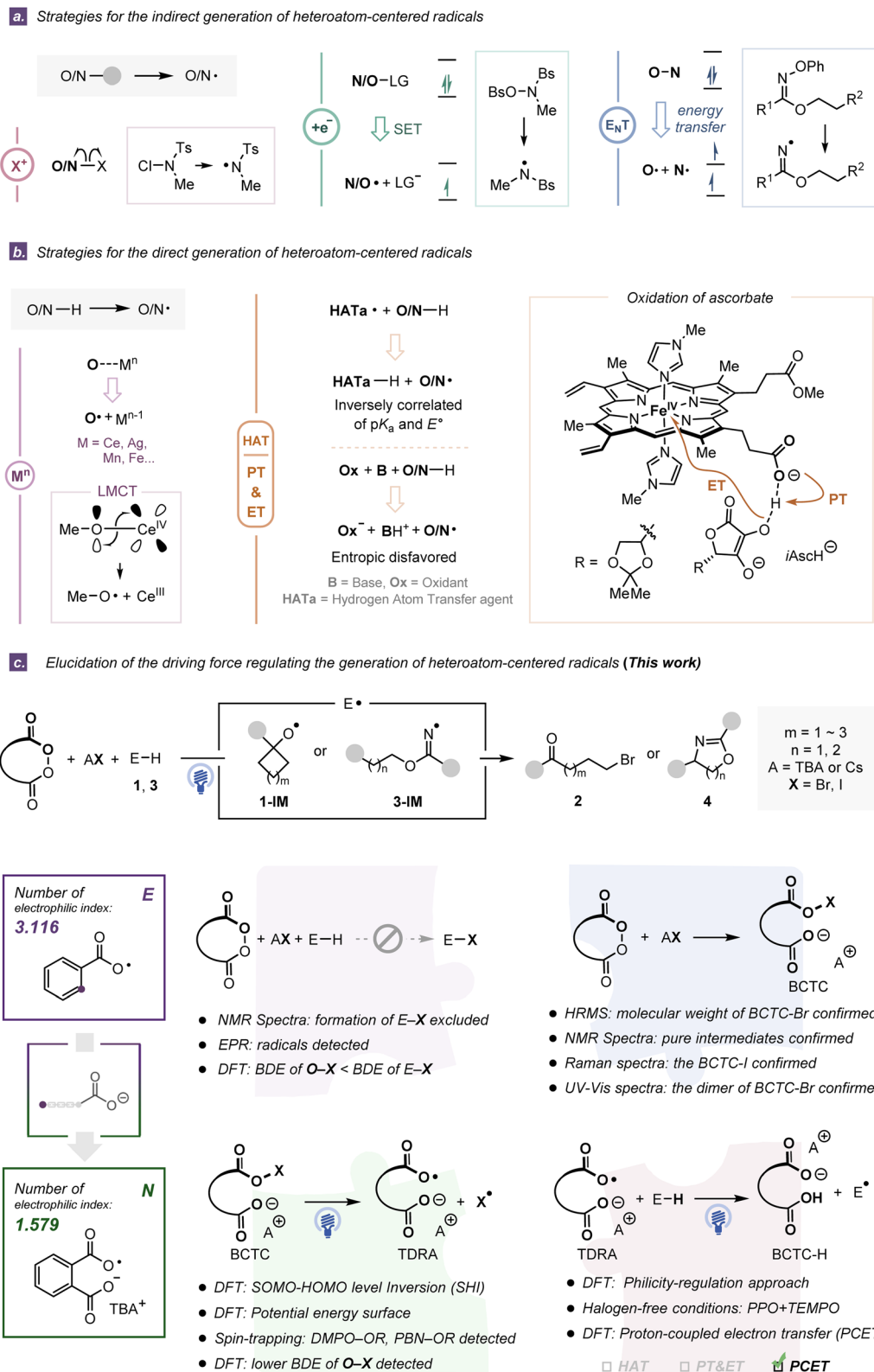
Fig. 1 (a) Strategies for the indirect generation of heteroatom-centered radicals. (b) Strategies for the direct generation of heteroatom-centered radicals. (c) Critical experimental and theoretical studies for the TDRA-mediated generation of heteroatom-centered radicals through the philicity-regulation approach and PCET step.
