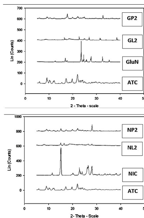
Figure 7. PXRD pattern of pure ATC, atorvastatin cocrystals with different cofomers and their physical mixtures.
