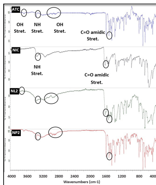
Figure 6. FT-IR spectra of pure ATC, nicotinamide (NIC), NL2 cocrystals (1:3, drug: NIC) prepared by SDG method, and NP2 physical mixture (1:3, drug: NIC).
