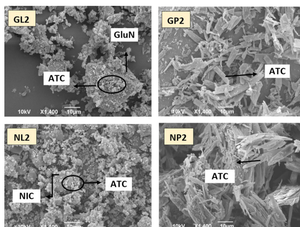
Figure 8. SEM photographs of atorvastatin cocrystals with different coformers and their physical mixtures..
