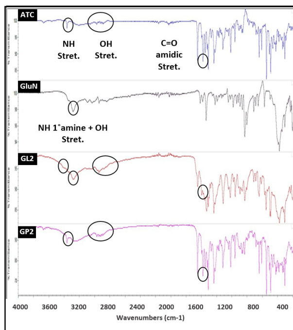
Figure 5. FT-IR spectra of pure ATC, glucosamine (GluN), GL2 cocrystals (1:3, drug: GluN) prepared by SDG method, and GP2 physical mixture (1:3, drug: GluN).
