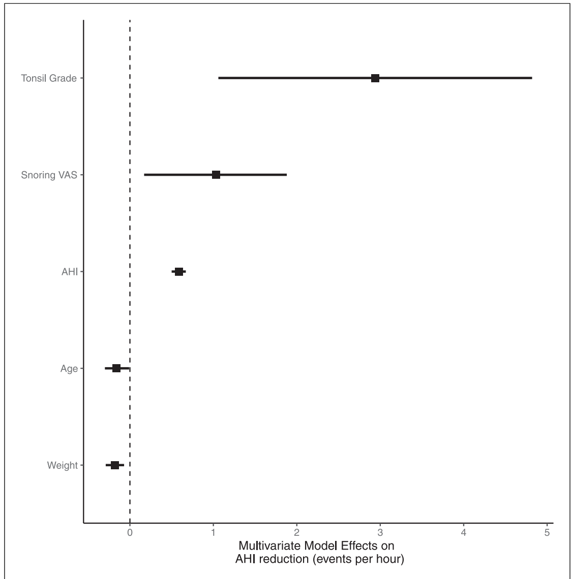
Fig. 1. Effects of different factors on AHI reduction are visualized in a forest plot with squares indicating the estimate and bars the 95% confidence intervals for a multivariate model.
