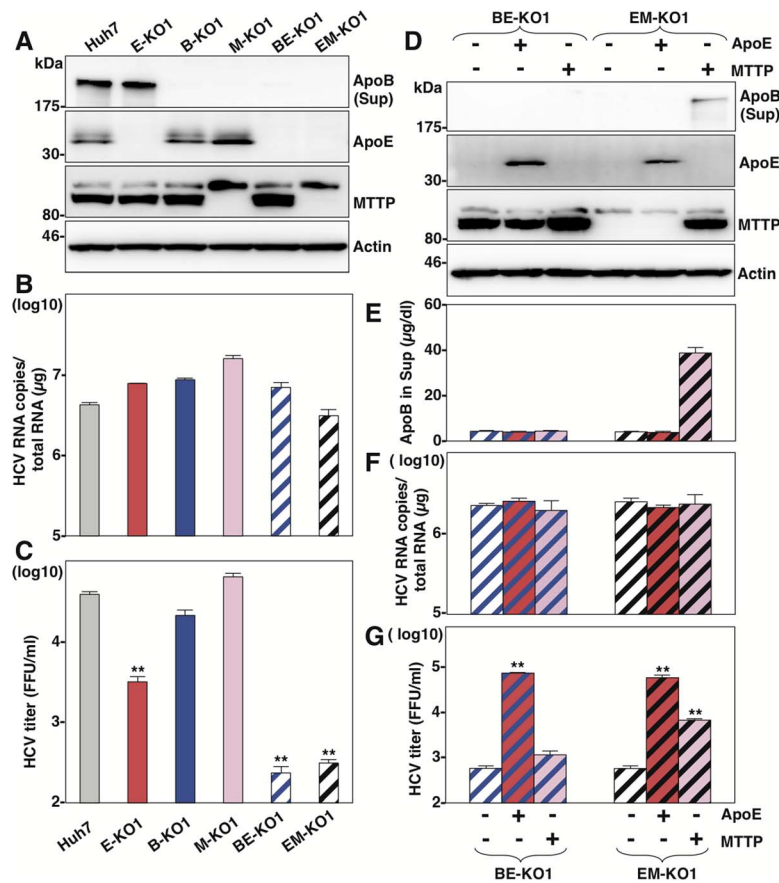
Figure 3. MTTP participates in the formation of infectious HCV particles through the maturation of ApoB. (A) Expressions of ApoB, ApoE and MTTP in Huh7, B-KO1, M-KO1, E-KO1, BE-KO1 and EM-KO1 cells were determined by immunoblotting analysis. Cells were infected with HCVcc at an MOI of 1, and intracellular HCV RNA (B) and infectious titers in the supernatants (C) were determined at 72 h post-infection by qRT-PCR and focus-forming assay, respectively. The expressions of ApoB, ApoE and MTTP in BE-KO1 and EM-KO1 cells with/without expression of ApoE or MTTP by lentiviral vector were determined by immunoblotting (D) and ELISA (E). Cells were infected with HCVcc at an MOI of 1, and intracellular HCV RNA (F) and infectious titers in the supernatants (G) were determined at 72 h post-infection by qRT-PCR and focus-forming assay, respectively. doi:10.1371/journal.ppat.1004534.g003
