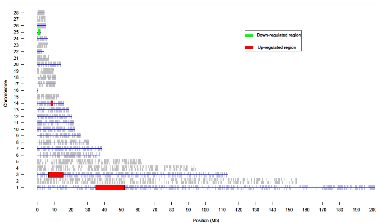
Figure 2 Differentially expressed chromosomal regions for contrast MM8-PM8. This figure showed the differentially expressed chromosomal regions for MM8.PM8 contrast ( q -value < 0.01 ). In total three regions were up-regulated and one region was down-regulated. Red showed the up-regulated chromosomal regions, and Green showed the down-regulated regions.
