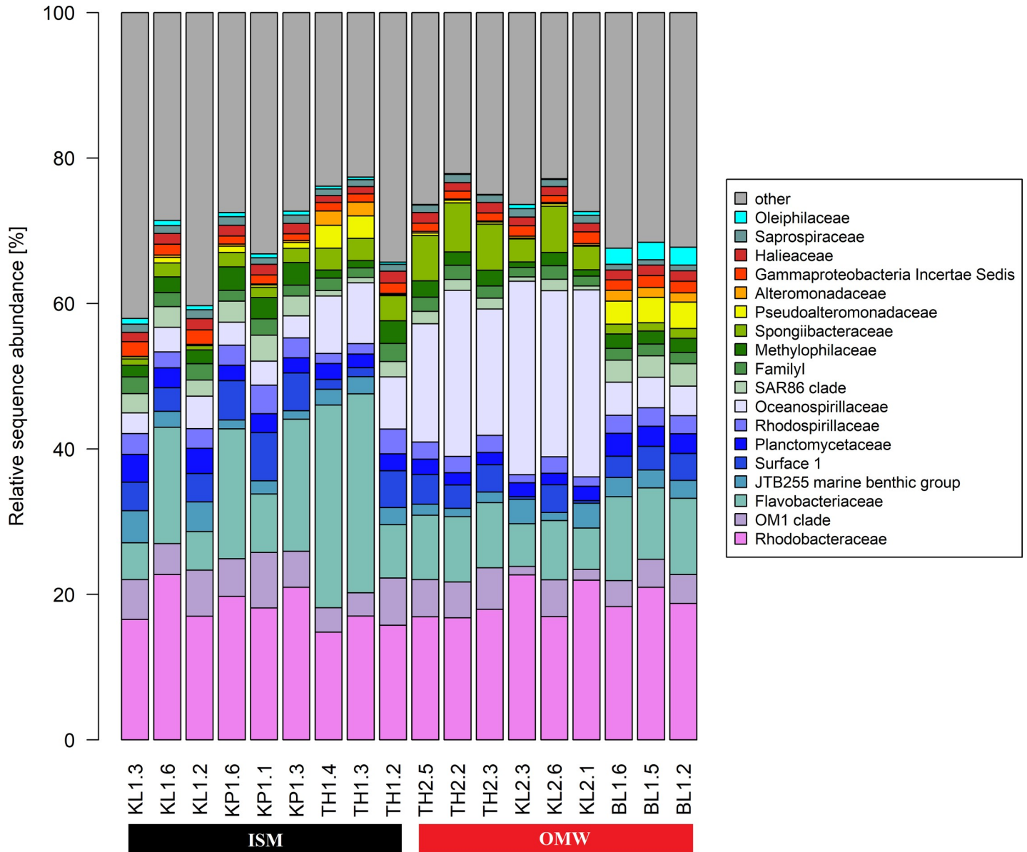
Fig 4. Taxonomic composition of dominant bacterial taxa on family level across eighteen samples under sites ISM and OMW (nine samples each). Ten (10) most abundant bacterial families for each of the samples were reported here and rests less dominant members are label as “other”.
