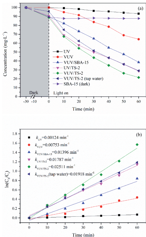
Fig. 8 Time course of UDMH concentration in different process (a) and rate constant of UDMH degradation (b). [\text{UDMH}]_0 = 100 \text{ mg L}^{-1} , \text{pH}_0 = 9.0 , T = 30^\circ \text{C} .
