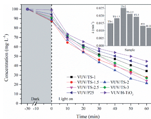
Fig. 9 Time course of UDMH concentration over \text{TiO}_2/\text{SBA-15} with different Ti contents in VUV process, with the rate constants (inset). [\text{UDMH}]_0 = 100 \text{ mg L}^{-1} , \text{pH}_0 = 9.0 , T = 30^\circ \text{C} .
