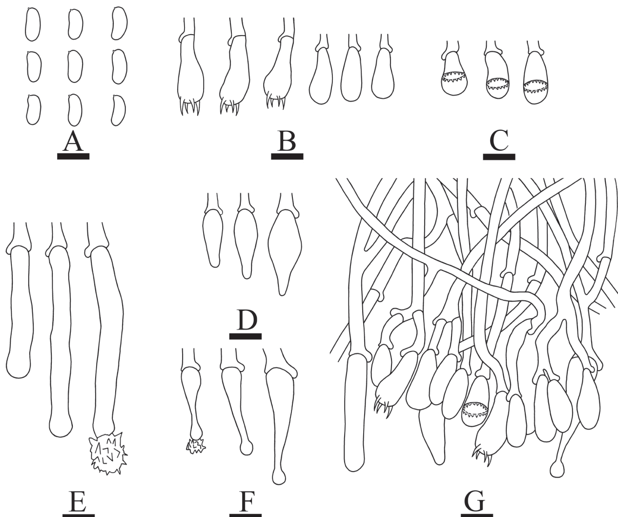
Figure 12. Microscopic structures of Peniophorella albohymenia (holotype, CLZhao 33187) A basidiospores B basidia and basidioles C stephanocyst D fusiform cystidia E cylindrical cystidia F capitate cystidia G a section of the hymenium. Scale bars: 10 \mu\text{m} ( A–G ).
