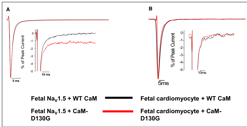
Figure 1. Long QT syndrome (LQTS) CaM mutation effects on persistent Na current are limited to a single splice variant of Na v 1.5 and a single CaM mutation. A, CaM-D130G evoked increased persistent sodium current with fetal Na v 1.5. Averaged tetrodotoxin-sensitive currents were normalized to the peak current measured at -30 mV during a 200-ms depolarization recorded under high intracellular Ca 2+ concentration (see Methods). The inset represents the same data plotted on an expanded vertical scale. Summary data are provided in Table 1. B, CaM-D130G has no significant effect on persistent Na current in fetal ventricular cardiomyocytes. Tetrodotoxin-sensitive currents were normalized to the peak current measured at -30 mV during a 300-ms depolarization recorded under high intracellular Ca 2+ concentration (see Methods). The inset represents the same data plotted on an expanded vertical scale. CaM indicates calmodulin; WT, wild type.
