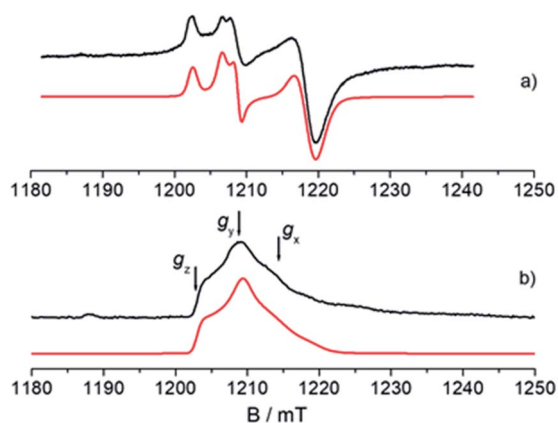
Fig. 2 Experimental (black) and simulated (red) Q-band EPR spectra of \text{CpTiCl}_3 after reaction with MMAO. (a) CW spectrum recorded with experimental parameters: temperature = 50 K, \text{mw}_{\text{frequency}} = 33.7 GHz, \text{mw}_{\text{power}} = 1 mW. The simulated spectrum is the sum of the Ti-H and Ti-R components, with relative weight 35 : 65. (b) Two-pulse ESE-EPR spectrum recorded with experimental parameters: temperature = 50 K, \text{mw}_{\text{frequency}} = 33.7 GHz, interpulse delay = 200 ns. The simulated spectrum only accounts for the Ti-H component. Simulation parameters are summarized in Table 1. Arrows indicate the magnetic field settings at which Davies ENDOR and HYSCORE experiments were performed.
