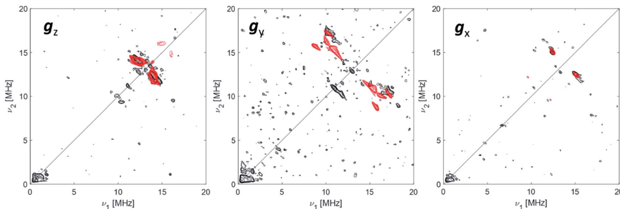
Fig. 4 ^{27}\text{Al} orientation selective Q-band HYSCORE spectra (black traces) and simulated spectra (red traces) of Ti-H at the three canonical positions of the EPR spectrum (as indicated by arrows in Fig. 2). The simulations correspond to a |A|^{27}\text{Al} = [2.0, 8.0, 1.0] MHz with Euler angles = [0, 0, 10]^\circ and nuclear quadrupole parameters e^2Qq/h = 18 MHz, \eta = 0 with Euler angles = [0, 0, 0]^\circ . Experimental conditions: temperature = 50 K, \text{mw}_{\text{frequency}} = 33.7 GHz, \pi/2 pulse = 16 ns, \pi pulse = 32 ns. Both experimental and simulated spectra are the sum of two spectra recorded with two different \tau values, which were summed together after Fourier transform. The following interpulse delays were used: \tau = 100 and 150 ns ( g_z ), \tau = 100 and 148 ns ( g_y ), and \tau = 110 and 148 ns ( g_x ).
