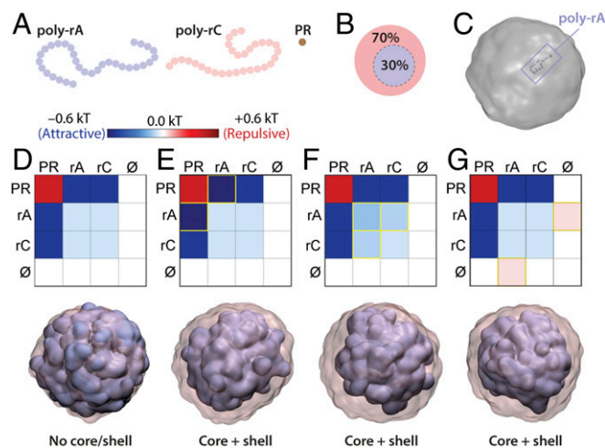
Fig. 5. Core–shell multilayered condensates can be formed via several distinct mechanisms. ( A ) Schematic of the molecular entities included in simulations based on the coarse-grained model that includes poly-rA, poly-rC, and PR. ( B and C ) Simulations are run with 70:30 split of poly-rC–poly-rA and give rise to droplets that are significantly larger than individual polymers. ( D–G ) A suitable interaction table defines the attractive and repulsive interactions between individual beads. These effective pairwise interactions represent the cumulative interplay among all bead–bead and bead–solvent interactions. Yellow boxes highlight differential values compared with D . When poly-rA and poly-rC are equivalent to one another, a single well-mixed droplet is formed (in D ). ( E ) If poly-rA–PR interaction is stronger than poly-rC–PR interaction, ( F ) if poly-rA–poly-rA interaction is stronger than poly-rC–poly-rA interaction which, in turn, is stronger than poly-rC–poly-rC interaction, or ( G ) if poly-rA–solvent is more repulsive than poly-rC–solvent, then topologically equivalent multilayered condensates are formed. Experimental data suggest that all three mechanisms may occur, to varying degrees.
