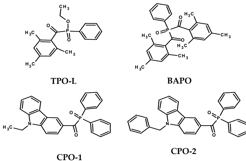
Figure 1. Chemical formula of the phosphine derivatives studied in this article.
