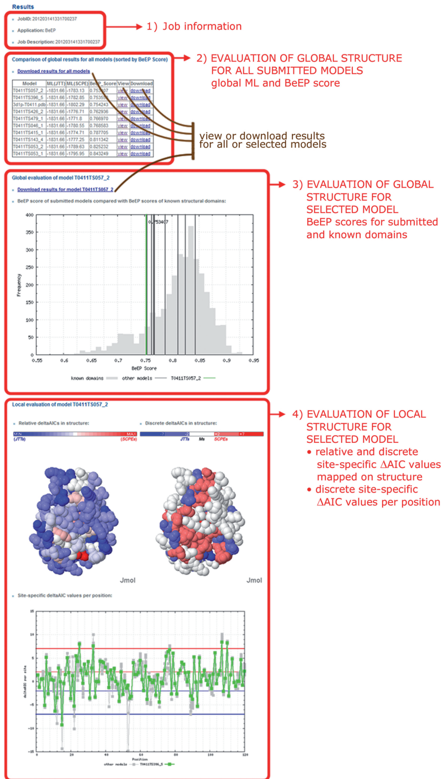
Figure 4. BeEP Server output explanation. The red boxes indicate different sections in the output. 1) Job information. The JobID can be used to retrieve results after the run has finished. 2) Table summarizing results of the global assessment of submitted protein structure models. For each submitted model, the table shows the global ML values obtained with the JTT general substitution model and the SCPE site-specific substitution model, together with the BeEP score on which the table is ranked. Links are provided to download a compressed file with all the results generated by the run, both for the individual models and for the complete dataset, or to load the results for a selected model. 3) BeEP score of all submitted models plotted on top of the distribution of BeEP scores for PDB structures of known domains. The selected model is displayed in green. The BeEP scores of known domains are provided as a reference, with good structure models expected to tend to the left (low) end of the distribution. 4) Different representations of the selected model based on the local \Delta AIC values. Site-specific scores are mapped on the structure in two different scales: the discrete colouring is useful for spotting SCS while the relative colouring can point to structurally conserved patches. A plot of site-specific \Delta AIC values per position helps to identify contiguous regions of the protein subjected to structural constraints. The reference horizontal lines are coloured according to the scale of discrete \Delta AIC values.
