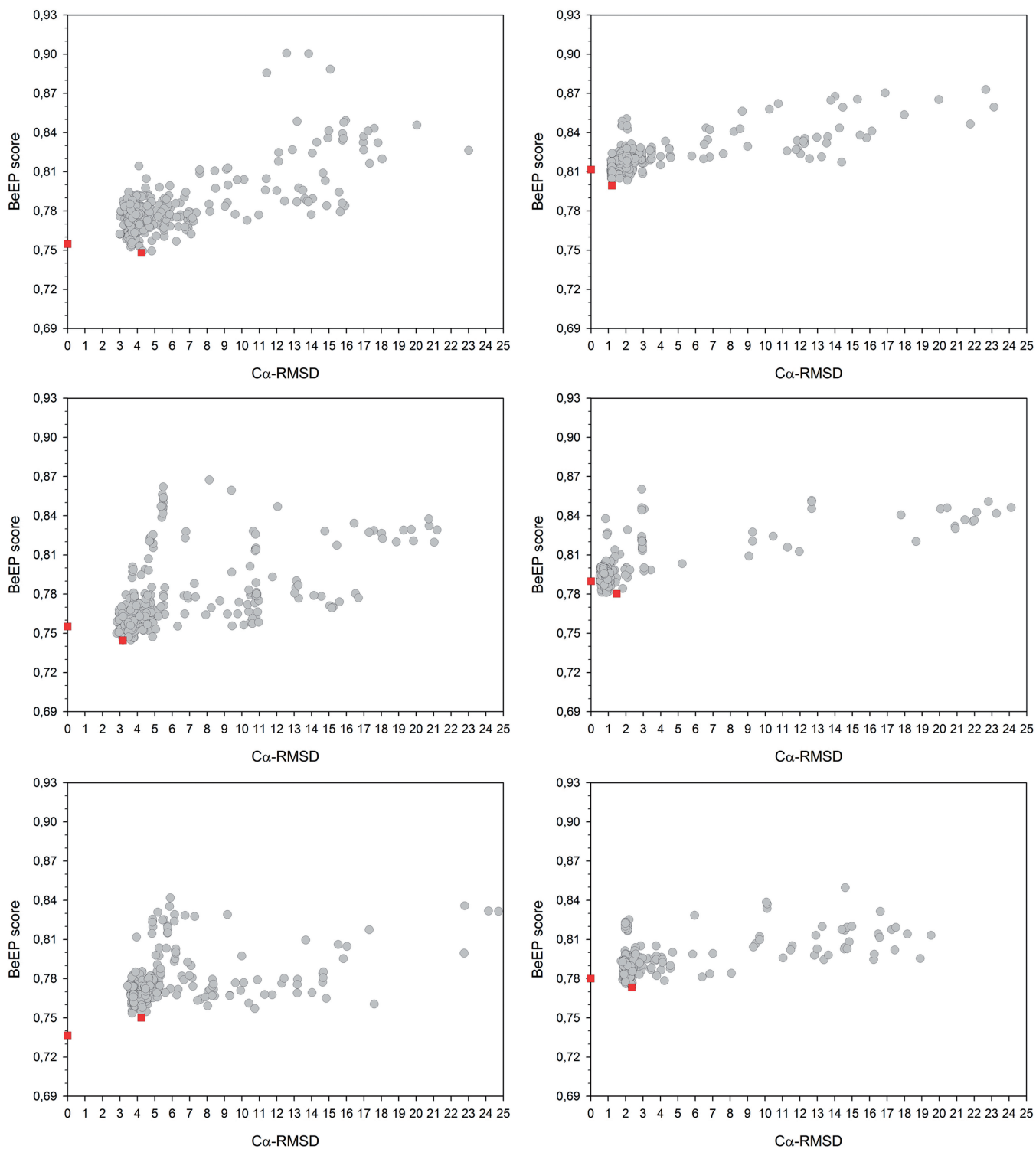
Figure 2. BeEP score versus C\alpha -RMSD to target protein for all structural models in six example sets selected from CASP8 targets (from left to right and top to bottom: T0411, T0418_D1, T0420, T0426, T0427_D2, T0506_D1). Each grey circle corresponds to a decoy model. The target structure (at C\alpha -RMSD = 0) and the best decoy are shown in red squares.
