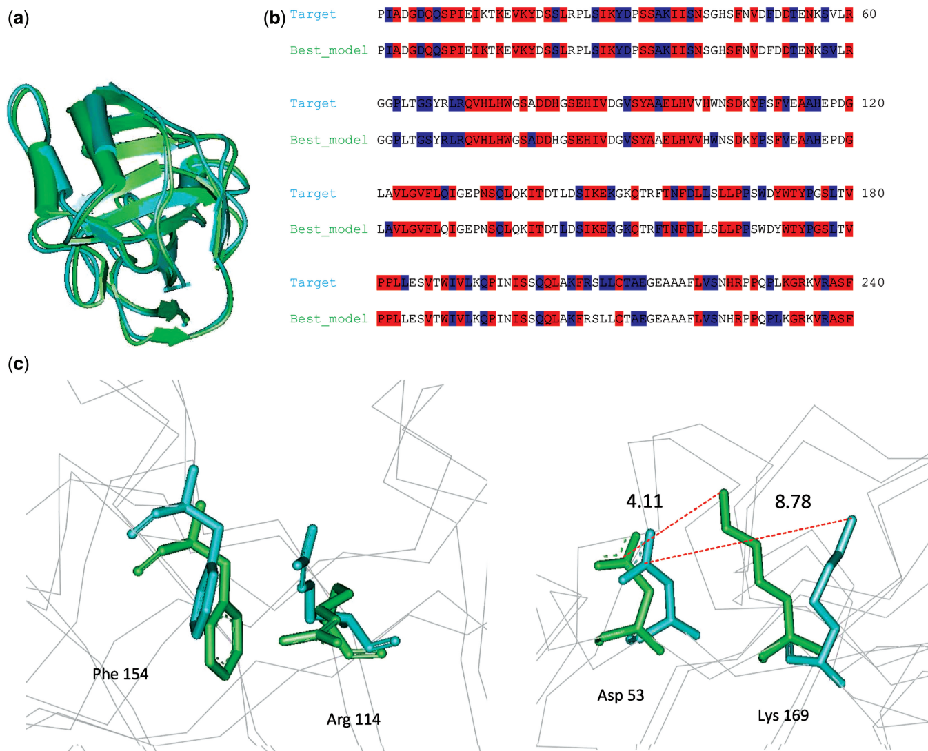
Figure 3. Slight variations in residue environments can change the BeEP score and increase the discrimination of decoys. In panel (a), we show the structural alignment between target structure T0426 (cyan) and the best decoy (light green) according to BeEP, which is ranked better than the target itself (see also Figure 2). Structural variations between target and best decoy produce changes in physicochemical environments of the residues favouring SCPE or JTT models. Derived SCPE (in red) and JTT (blue) sites are displayed in panel (b). The number of SCS in the target and in the best decoy is 106 and 103, respectively. However, the BeEP score accounts for the difference in the likelihood between SCPE and JTT models in SCS sites (see BeEP score equation in Methods). In panel (c), we show two examples of how different residues rearrangements could favour the occurrence of given residues and then increase SCPE likelihood in the best decoy against the target structure. In panel c, left, a pair of arginine (Arg) and phenylalanine (Phe) show a better geometry to form a pi-cation interaction in the best decoy. In panel c, right, the distance to establish a Coulomb interaction between aspartate (Asp) and lysine (Lys) residues is better in the best decoy than in the target structure.
