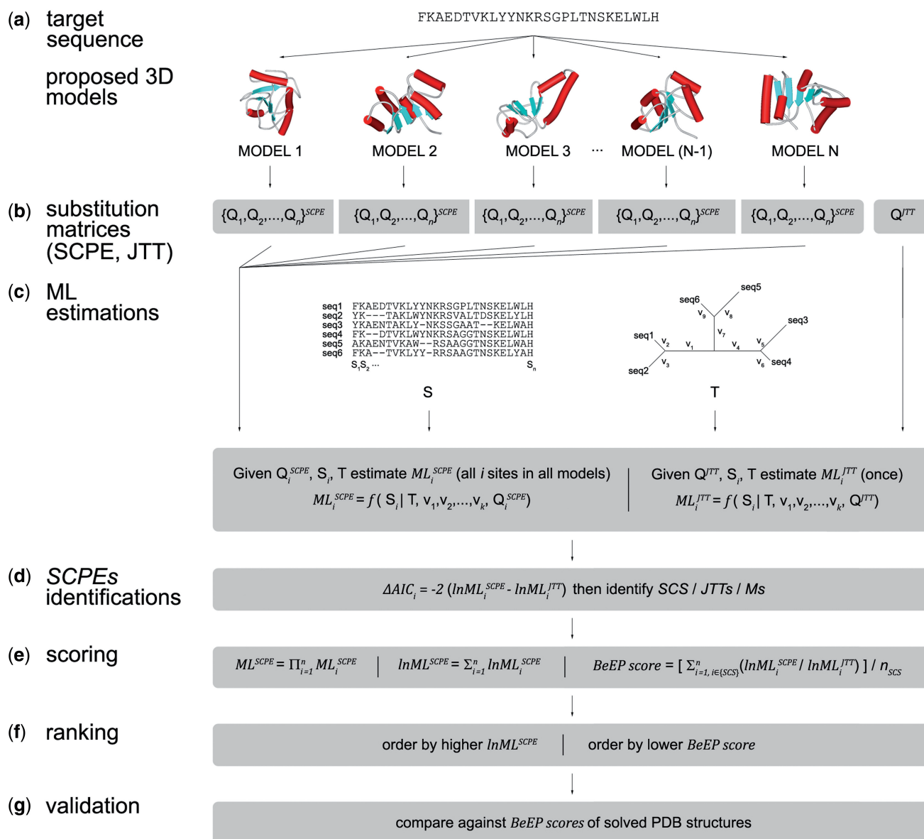
Figure 1. Schematic representation of the BeEP workflow. Given a protein of interest with length n and different proposed structural models (a), the SCPE is used to derive a set of site-specific substitution matrices for each model (b). Using ML estimations, it is possible to evaluate the correlation of each substitution matrix with the information contained in a sequence alignment S of homologous proteins by optimizing the branch lengths on a corresponding phylogenetic tree T (c). The site-specific ML values obtained using SCPE matrices are compared with the ML values calculated with the substitution matrix Q^{JTT} of the unconstrained model JTT to identify sites subjected to structural constraints (SCS) (d). BeEP scores are derived from the site-specific ML (e) values and the set of structural models can be ranked through the comparison of these scores (f). Further validation of native-like models can be achieved by comparison with the BeEP scores of known structures (g).
