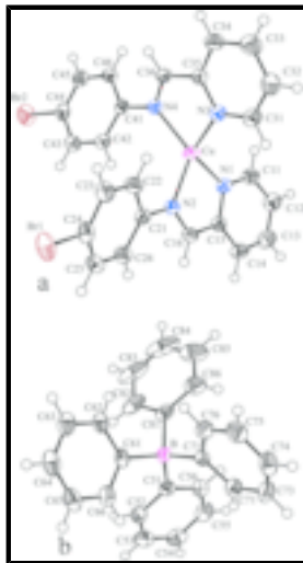
Fig. 1. Crystal structure of the cation (a) and the anion (b) with labeling and thermal ellipsoids drawn at 50% the probability level. Hydrogen atoms are shown as spheres of arbitrary radius.
