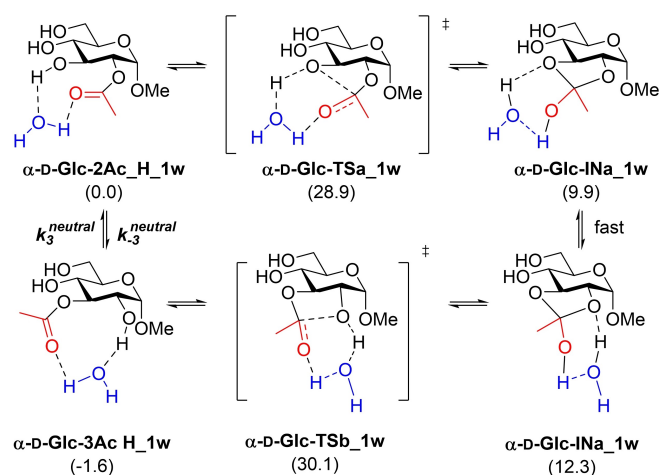
Scheme 4. Acetyl group migration under neutral conditions mediated by one molecule of water. Relative energies (kcal/mol) calculated at m062x/cc-pvtz/SMD = water//m062x/6-31 + G(d,p)/SMD = water level of theory are given in brackets.
