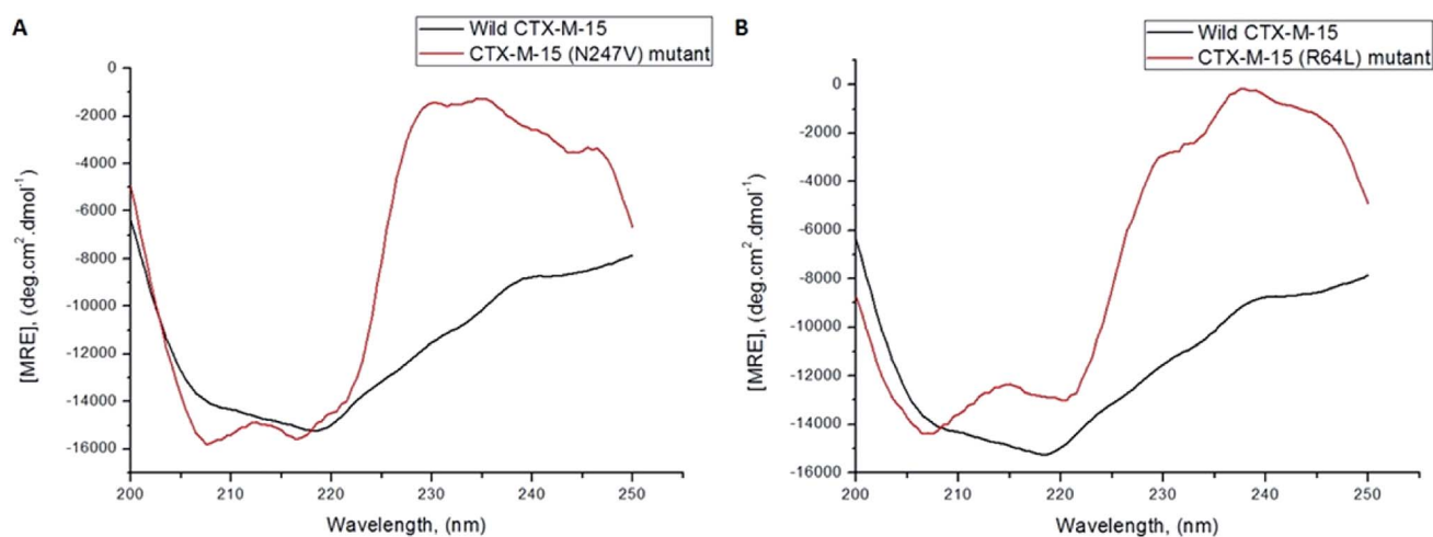
Fig. 3 Panel (A) shows the far-UV CD spectra of 5 \mu M of the CTX-M-15 enzyme and 5 \mu M of the CTX-M-15 (N247V) mutant enzyme. Panel (B) shows the far-UV CD spectra of 5 \mu M of the CTX-M-15 enzyme and 5 \mu M of the CTX-M-15 (R64L) mutant enzyme. The experiment was carried out at 298 K in the presence of pH 7.4 sodium phosphate buffer.
