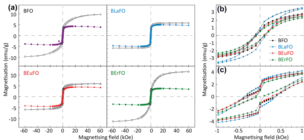
Figure 5. (a) M-H curves of neat and doped BFO, measured at 300 K (coloured—filled symbols) and 2 K (black—open symbols), (b) enlarged M-H curves of neat and doped BFO measured at 300.0 K and (c) 2.0 K.
