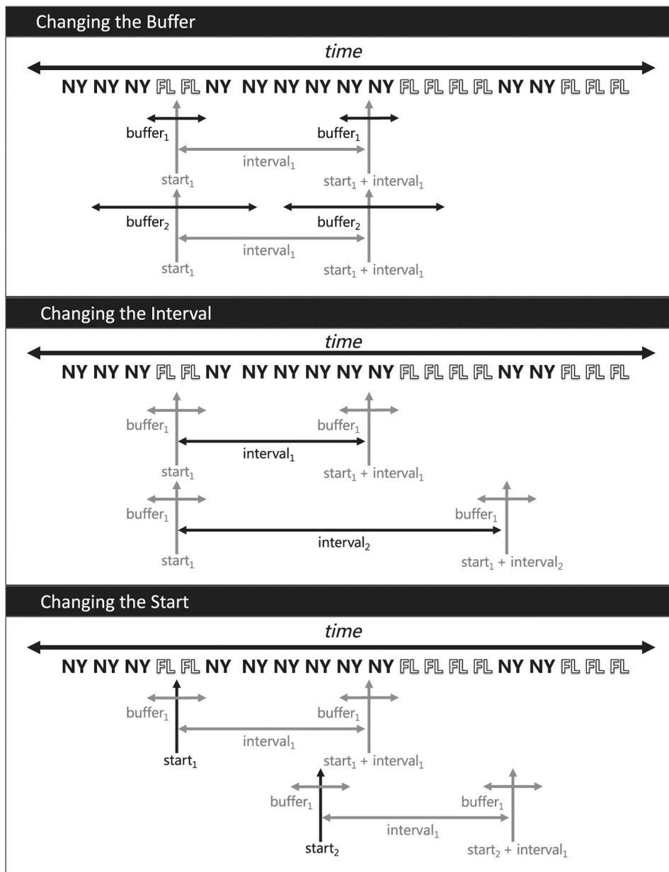
Fig. 1. Three interlocking but distinct dimensions of migration measurement: start, buffer, and interval. By changing one while holding the other two fixed, we can assess how migration estimates are affected by seasonality (start), residency criteria (buffer), and cumulative exposure to migration risk (interval).
