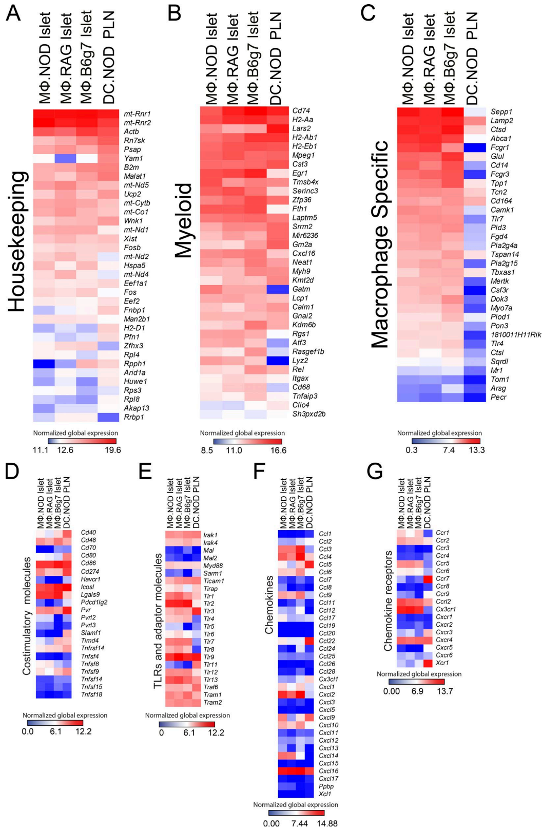
Figure 1. Transcriptional profiling of islet-resident macrophages. Top expressed housekeeping (A) and myeloid (B) genes from NOD, NOD.Rag1 -/- , and B6.g7 islet macrophages and DCs. Macrophages and DCs were isolated as indicated in Fig. S1. (C) Core macrophage-specific gene signature (as defined by Gautier et al., 2012), distinguishing macrophages from DCs. Expression of costimulatory genes (D), genes encoding TLRs and adaptors (E), chemokines (F),
