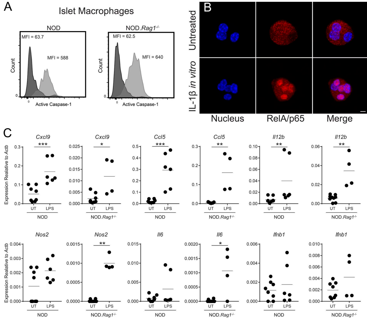
Figure 6. Inflammatory status of islets before and after treatment with LPS. (A) NOD or NOD.Rag1 -/- mouse islet macrophages were isolated and stained with the intracellular caspase-1 substrate FAM FLICA YVAD-FMK. The black histograms are gated on the CD45-negative fraction of the islets, and the gray histograms are gated on macrophages as in Fig. S1. Mean fluorescent intensity (MFI) is indicated on the graphs. MFIs for active caspase-1 ranged from 62.5–102 (mean 72.2) for the CD45 neg population and from 388–884 (mean 625) for the F4/80 + population. Data are representative of two or three independent experiments per group. (B) Islets from 6-wk-old NOD mice were isolated, dispersed, and cultured overnight in chamber slides in the absence or presence of IL-1β. Cells were then stained with DAPI (blue) and anti-RelA/p65 (red). Cells were imaged by confocal microscopy. Bar, 4 μm. Image is representative of three independent experiments. (C) Expression of inflammatory gene transcripts in macrophages isolated from islets of mice intravenously injected with LPS. The indicated mice were treated with either PBS (UT) or LPS IV (LPS). Then, islet macrophages were flow-sorted, RNA was isolated, and qRT-PCR was performed on the indicated markers. Each symbol represents one individually sorted sample. Horizontal bars show the mean. Significance was tested using the Mann-Whitney U test. *, P < 0.0332; **, P < 0.0021; ***, P < 0.0002. Graphs show all the data from at least three independent experiments performed in duplicate for each condition.
