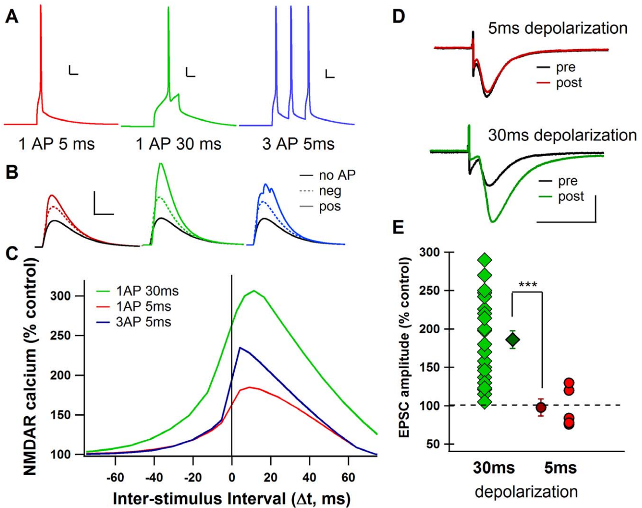
Figure 2. STDP protocol type changes calcium influx through NMDAR. A. Model traces showing each STDP protocol. Scale bars: 10 mV vertical, 10 ms horizontal. B. NMDAR-mediated calcium during positive (solid color line) and negative (dotted color line) \Delta t compared to calcium through NMDA during synaptic stimulation only (No AP, solid black line). Scale bars: 2 \mu\text{M} [\text{Ca}^{2+}] vertical, 50 ms horizontal. C. Model calcium curves showing change in peak NMDAR calcium as a percentage of control (synapse stimulation with no AP). Spines stimulated are 40 \mu\text{m} from the soma. D. Example single experiments showing tLTP in response to 30 ms depolarization STDP, but not to 5 ms depolarization STDP. pre = average of baseline EPSCs prior to STDP; post = average of EPSCs around 60 minutes after STDP. Scale bars: 100 pA vertical, 20 ms horizontal. E. All experimental data points approximately 60 minutes after STDP protocol application as % of baseline. 5 ms depolarization STDP failed to induced significant tLTP when compared to 30 ms depolarization STDP. (***) = p < 0.0001 . doi:10.1371/journal.pcbi.1002493.g002
