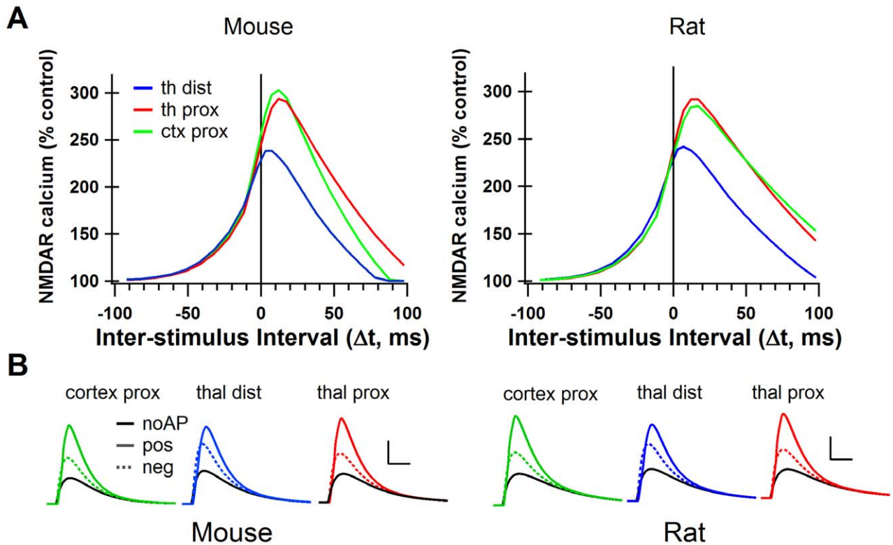
Figure 6. The cortico-striatal and thalamo-striatal synapses onto MSPNs have different synaptic characteristics. A. Peak NMDAR calcium curves from simulations using cortico-striatal and thalamo-striatal parameters from mouse striatum (Ding et al., 2008) and from rat striatum (Smeal et al., 2008). Cortico-striatal curve for mouse is the same as the green trace in figure 2C. B. NMDAR-mediated calcium for positive ( \Delta t = +11 ms, solid color), negative ( \Delta t = -12 ms, dotted color) and no AP control conditions (solid black) under cortico-striatal and thalamo-striatal conditions in mouse and rat. Scale bars: 2 \mu\text{M} [ \text{Ca}^{2+} ] vertical, 50 ms horizontal. thal dist = thalamo-striatal synapses stimulated on tertiary dendritic spines, thal prox = thalamo-striatal synapses stimulated on secondary dendritic spines. cortex prox = cortico-striatal synapses stimulated on secondary dendritic spines.
