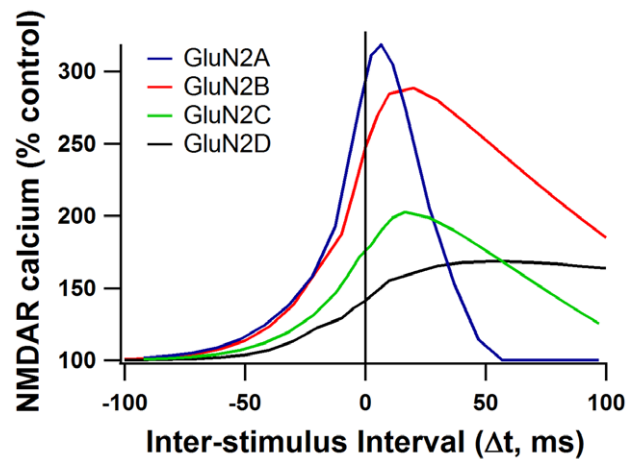
Figure 3. Calcium curves for different GluN2 subunit containing NMDARs. Dependence of NMDAR-mediated calcium on AP timing is different for each GluN2 subunit. Normalized peak NMDAR calcium is plotted for each AP timing interval ( \Delta t ) using the 30 ms STDP protocol. Spines stimulated are 40 \mu\text{m} from the soma. doi:10.1371/journal.pcbi.1002493.g003
