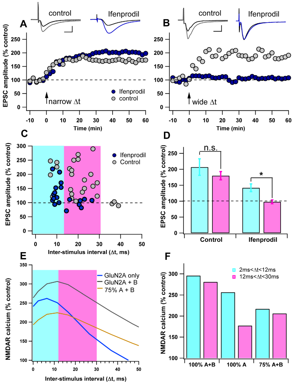
Figure 4. GluN2B broadens the STDP curve. A–B. Inhibition of GluN2B restricts the time window of tLTP induction. Representative experiments illustrate the time course of synaptic efficacy changes induced by pre-post pairings in control aCSF and in the presence of ifenprodil (10 \mu M). Insets: averaged EPSCs before (black) or after (grey: control; blue: ifenprodil treatment) STDP. Scale bars 100 pA vertical, 10 ms horizontal. A . Example experiments showing tLTP induced by narrow AP timing intervals ( 0 < \Delta t < 12 ms) in control and ifenprodil conditions. B . Example experiments showing tLTP is induced by wide AP timing intervals ( 12 < \Delta t < 30 ms) in control conditions, but not induced when GluN2B containing NMDARs were
