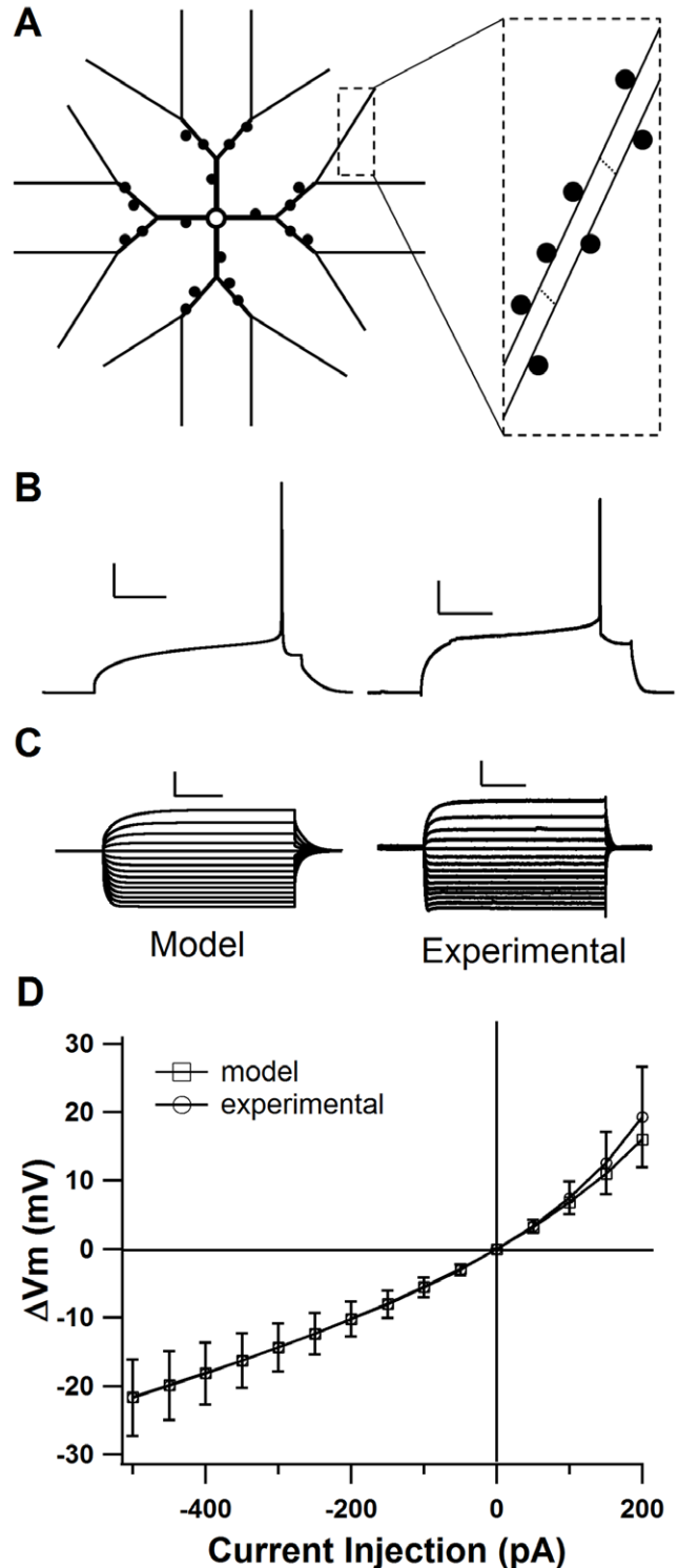
Figure 1. Model cell shows MSPN characteristics. A. Morphology of model MSPN (not to scale). Inset: tertiary dendrites have 11 segments each 36 \mu\text{m} in length. B. Comparison traces demonstrating latency to first AP in the model MSPN and an experimental whole-cell recording of a mouse MSPN. Both traces are a voltage response to current injection of 280 pA. Scale bars: 20 mV vertical, and 100 ms horizontal. C. Comparison current-voltage relationships ( -500 pA to 200 pA) for the model MSPN and an experimental recording demonstrating inward rectification. Scale bars: 10 mV vertical, and 100 ms horizontal. D. Current-voltage relationship for computational model compared with mean current-voltage relationship from 25 MSPNs of the mouse dorsal striatum. (See also Text S1: Supplemental Methods) Error bars \pm SD. doi:10.1371/journal.pcbi.1002493.g001
