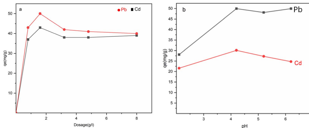
Fig. 9 (a) Effect of adsorbent dosage of \text{Fe}_3\text{O}_4\text{@NR-TMD-G1} ( T = 298 K, \text{pH} = 4.3 , initial concentration = 200 \text{mg L}^{-1} , contact time = 30 min) and (b) effect of pH on the adsorption of \text{Pb(II)} and \text{Cd(II)} ions ( T = 298 K, initial concentration = 200 \text{mg L}^{-1} , adsorbent = 0.08 g, contact time = 30 min).
