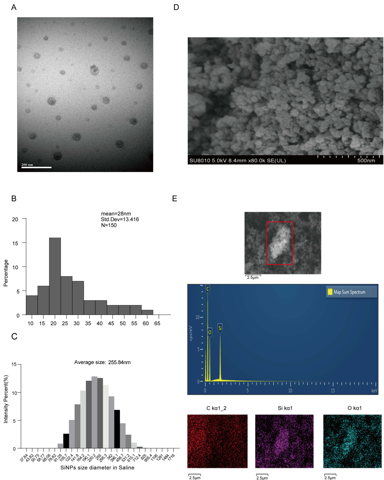
Figure 1 Characteristics of SiNPs used in this study. (A) SiNPs were detected by transmission electron microscopy. Scale bar, 200 nm. (B) ImageJ was used to measure the average size of 150 SiNPs in the TEM image, which was approximately 28 \pm 13.416 nm. (C) Dynamic light scattering (DLS) determined the hydrodynamic diameter of SiNPs used in this study, which was found to be 255.84 nm. (D) Scanning electron microscope image of SiNPs. Scale bar, 500 nm. (E) FE-SEM/EDS used to detect the major chemical elemental composition of SiNPs. Scale bar, 5 µm.
