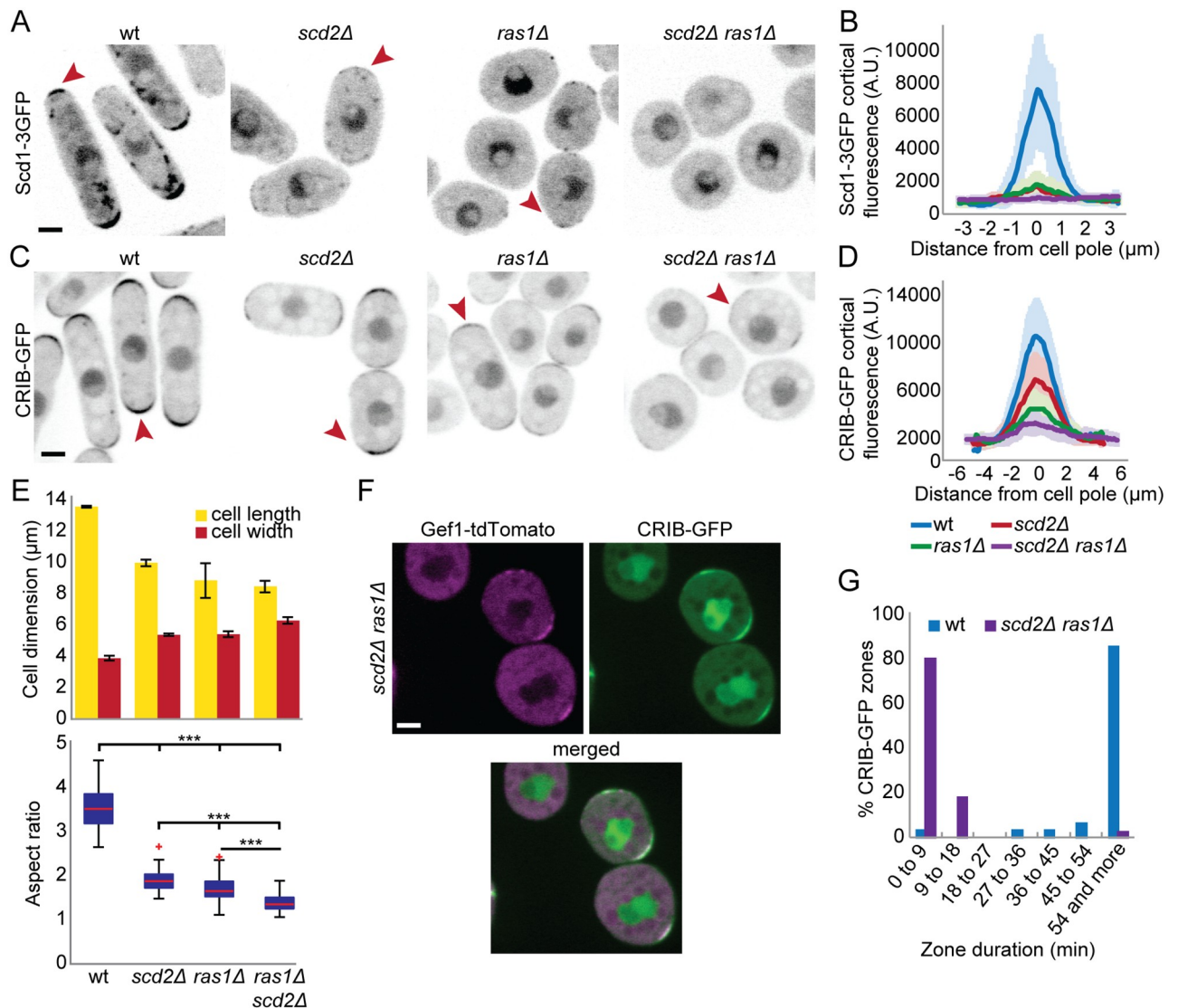
Fig 1. Ras1 and Scd2 cooperate for Scd1 recruitment to cell poles. (A–D) Localization of Scd1-3GFP (A–B) and CRIB-GFP (C–D) in wt, ras1Δ , scd2Δ , and ras1Δ scd2Δ cells. (A) and (C) show representative B/W inverted images; (B) and (D) show cortical tip profiles of Scd1-3GFP and CRIB-GFP fluorescence; n = 24 and 26 cells, respectively. Thick line = average; shaded area = standard deviation. (E) Mean cell length and width at division (top) and aspect ratio (bottom) of strains as in (C) ( n > 30 for 3 independent experiments). Bar graph error bars show standard deviation; box plots show the ratio between cell length and cell width. On each box, the central mark indicates the median; the bottom and the top edges indicate the 25th and 75th percentiles, respectively; the whiskers extend to the most extreme data points not considering outliers, which are plotted individually using the red “+” symbol. *** indicates 2.8e^{-90} \leq p \leq 1.9e^{-10} . (F) Colocalization of CRIB-GFP and Gef1-tdTomato in ras1Δ scd2Δ double-mutant cells. Bar = 2 \mu\text{m} . (G) Lifetime of CRIB-GFP cortical zones over 1 h, in wt and ras1Δ scd2Δ cells ( n = 32 and 39 zones respectively). All underlying numerical values are available in S1 Data. A.U., arbitrary units; B/W, black and white; wt, wild type.
