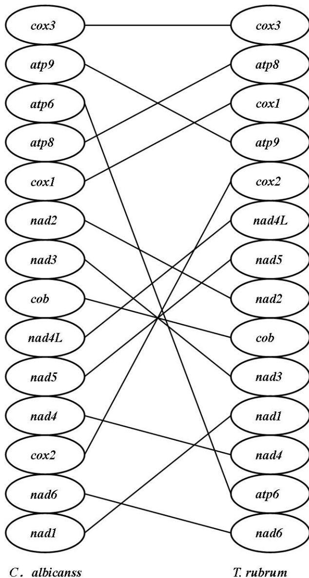
Figure 3 Comparison of the genomic organization of 14 protein-coding genes in T. rubrum and C. albicans (GenBank accession: NC_002653) mtDNAs.
