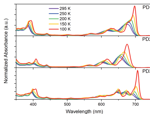
Fig. 4 Ground-state absorption spectra of dimers PD1 – 3 in MTHF at temperatures ranging from 295 to 100 K.
