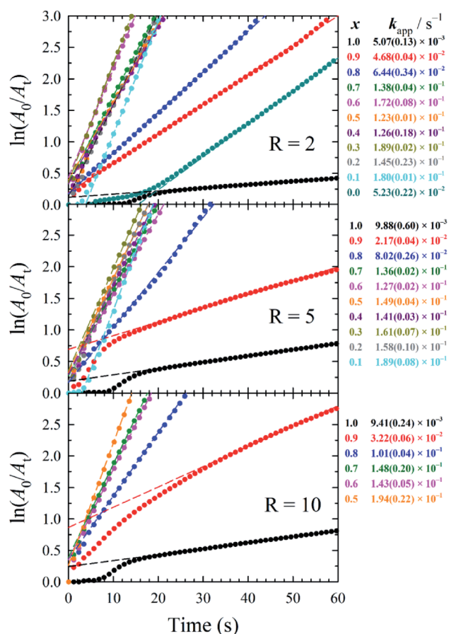
Fig. 3 Plots depicting the pseudo-first-order kinetics of 4-NP reduction and associated catalytic rates ( k_{\text{app}} ) using 5 d-old borohydride-stabilized \text{Au}_x\text{Ag}_{1-x} NP nanocatalysts ( R = 2, 5 , and 10 , top to bottom). Excluded x values for a particular R value indicate the observation of appreciable colloidal precipitation after aging for 5 d.
