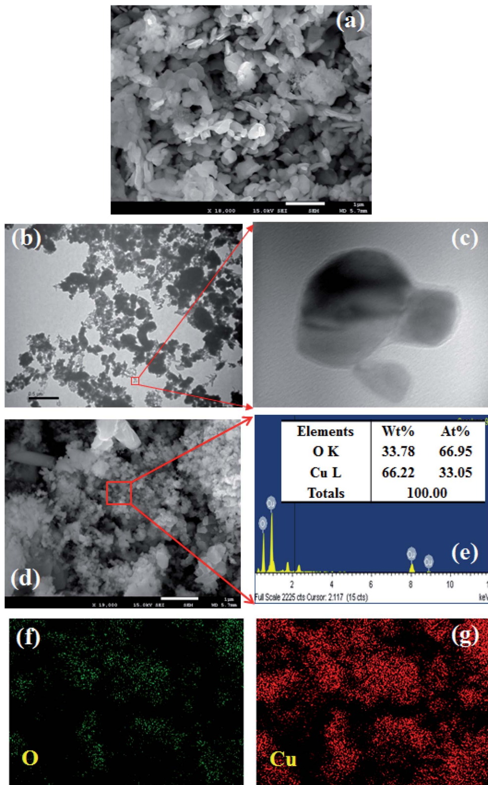
Fig. 2 Analyses of CuO NPs. (a) FESEM, (b and c) low to high magnified TEM images, (d and e) elemental analysis (inset: elemental compositions of O and Cu), and (f and g) elemental mapping of O and Cu.
