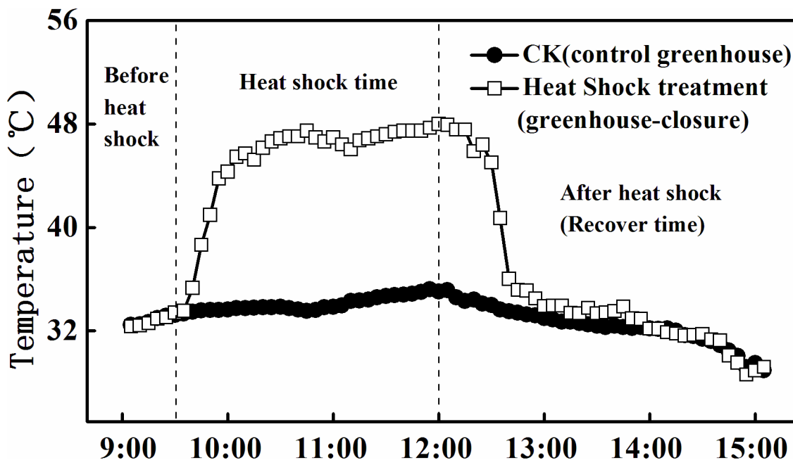
Fig 1. Temperature changes in heat shock treatment and control greenhouses.
