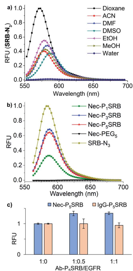
Fig. 2 Photophysical properties of SRB-N 3 and the resulting Ab-P n SRB probes. (a) Fluorescence spectra of SRB-N 3 (5 μM) in different solvents (λ ex = 530 nm). (b) Fluorescence spectra of Nec-P n SRB (100 nM) and SRB-N 3 (20 nM) in H 2 O (λ ex = 530 nm). (c) Fluorescence response of Nec-P 5 SRB/IgG-P 5 SRB (20 nM) in the presence of recombinant EGFR at different ratios (λ ex = 560 nm and λ em = 590 nm).
