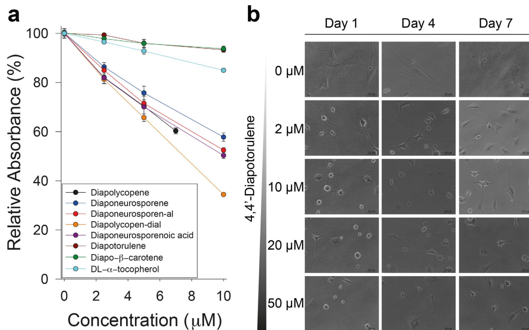
Figure 6. Comparison of DPPH scavenging activity of various C_{30} carotenoids and morphological changes of rBMSCs treated with varying concentrations of 4,4'-diapotorulene for 7 days. (a) DL- \alpha -tocopherol was used as a control antioxidant. Values are represented as the mean \pm SD from three independent experiments. (b) Cells were treated with varying concentrations of 4,4'-diapotorulene and observed under the microscope for 7 days. Scale bar represents 50 \mu m.
