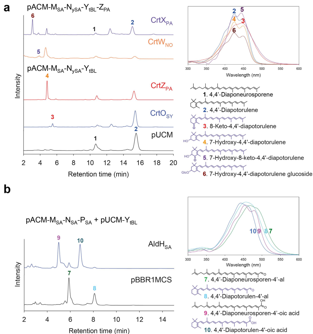
Figure 4. Analysis of C_{30} monocyclic carotenoids produced by engineered E. coli cells. (a) HPLC profiles of the C_{30} monocyclic carotenoids pathway reconstructed in E. coli expressing background pACM-M_{SA}-N_{ySA}-Y_{tBL} or pACM-M_{SA}-N_{ySA}-Y_{tBL}-Z_{PA} and C_{40} carotenoid modifying enzymes ( CrtX_{PA} , CrtW_{NO} , CrtZ_{PA} and CrtO_{SY} ). (b) HPLC profiles of the C_{30} monocyclic carotenoids pathways reconstructed in E. coli expressing pACM-M_{SA}-N_{SA}-P_{SA} with CrtY_{tBL} and AldH_{SA} . UV/Vis absorption spectra for compounds corresponding to individual peaks are shown in the upper-right panels. Identified carotenoid structures are shown in the lower-right panels.
