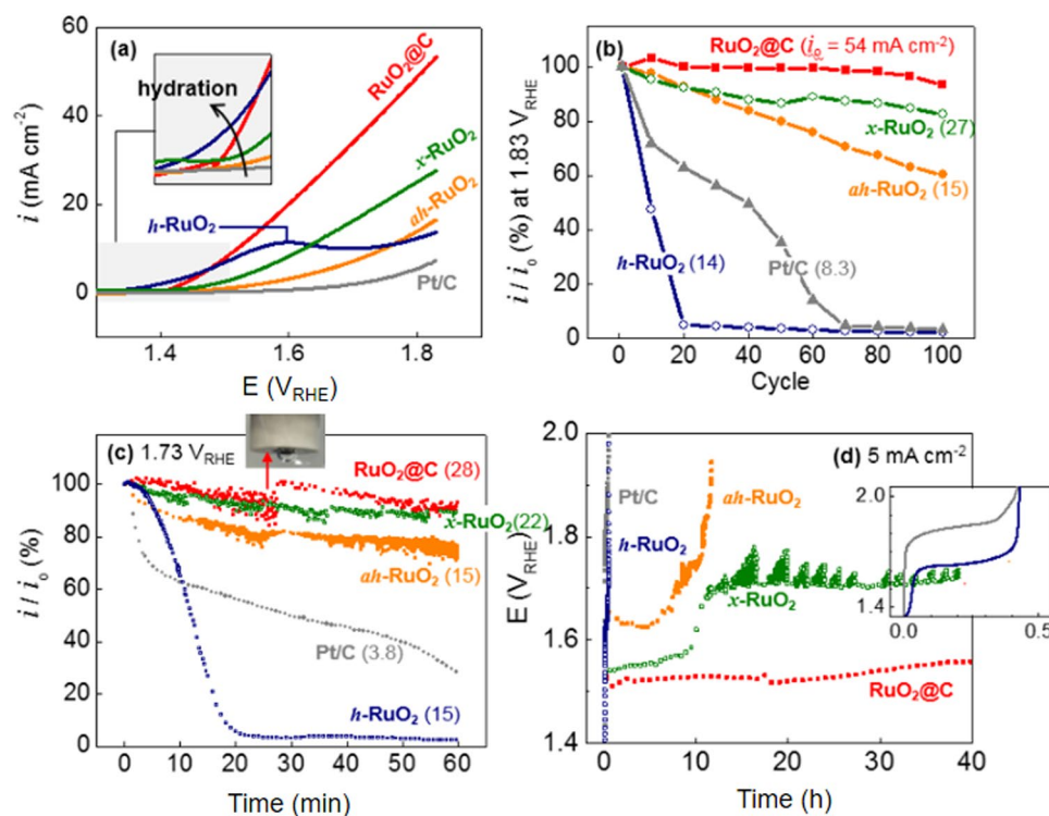
Figure 4. OER in N_2 -saturated 0.1 M KOH (aq). (a) OER polarization curves at 1,600 rpm for the first potential sweep cycles at 10 \text{ mV s}^{-1} . (b) OER current retention at 1.83 \text{ V}_{\text{RHE}} during repeated cyclic voltammograms. (c) Chronoamperometric stability of OER at 1.73 \text{ V}_{\text{RHE}} for 60 min in 0.1 M KOH. The initial currents are indicated next to the names of the catalysts. (d) Chronopotentiometric stability of OER at 5 \text{ mA cm}^{-2} for 40 h.
