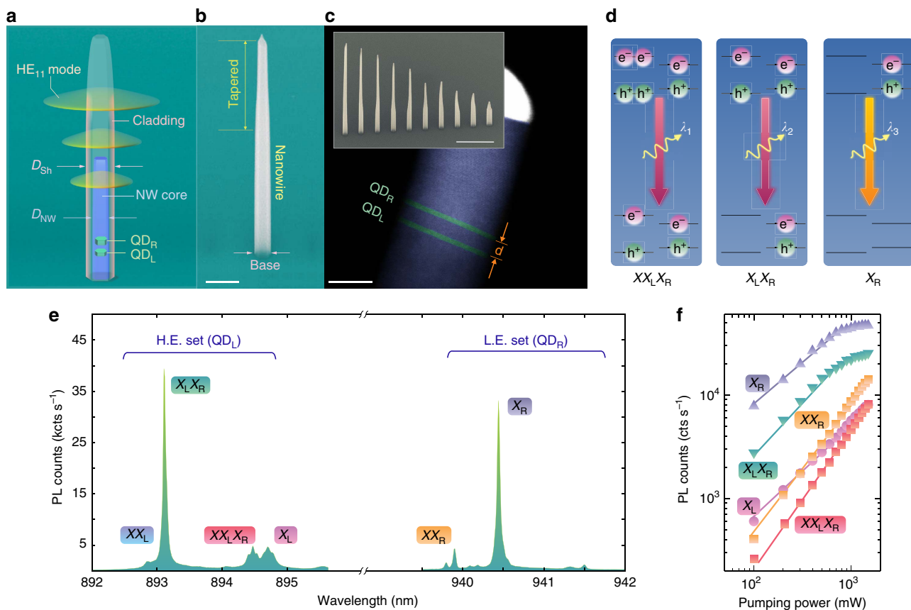
Figure 1 | Structure and spectrum of a nanowire-QDM. (a) Schematic of a quantum dot molecule (QDM) embedded inside a clad nanowire. The best suited nanowires consist of a thin core region D_{NW} = 18\text{--}20 nm surrounded by a thick InP cladding (shell) D_{Sh} = 250 nm that waveguides at least one principal optical mode at QDM emission wavelengths \approx 894 and \approx 940 nm. (b) False-coloured scanning electron microscopy image of a spatially isolated nanowire with hexagonal crosssection incorporating a single QDM. The scale bar is 500 nm. (c) False-coloured transmission electron microscopy image of an InP nanowire (core) grown on (111)B substrate in wurtzite phase embedding two In(As)P quantum dots separated by \approx 7 nm. The scale bar is 10 nm. Inset: The nanowires are site-controlled allowing excellent isolation of QDM spectrum from inhomogeneous broadening. The scale bar is 1 \mu m. (d) Triple sequential transitions: carrier configurations of high-energy (HE) triexciton, separated biexciton and low-energy (LE) exciton. (e) Optical spectrum of QDM comprising two prominent features at \approx 894 and \approx 940 nm. (f) photoluminescence intensity of the QDM resonances showing linear or superlinear dependence on the pump power.
