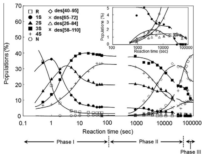
Fig. 9. A whole time course for oxidative folding of RNase A by using \text{DHS}^{\text{ox}} as an oxidant at pH 8.0 and 25 °C. Reaction conditions: [R]_0 = [\text{DHS}^{\text{ox}}]_0/3 = 48.0 \mu\text{M} for phase I, [R]_0 = [\text{DHS}^{\text{ox}}]_0/3 = 26.4 \mu\text{M} for phase II, [R]_0 = [\text{DHS}^{\text{ox}}]_0/3 = 17.0 \mu\text{M} for phase III. The relative populations of 1S, N, and des intermediates are expanded in an inset.
