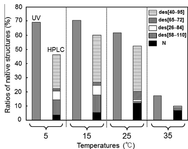
Fig. 6. Comparison of the ratios of native structure of RNase A estimated by UV measurement at 287 nm and those of the native state (N) and des intermediates at pH 8.0. Reaction conditions: [R]_0 = [\text{DHS}^{\text{ox}}]_0/3 = 25.1 \mu\text{M} at 5 °C, [R]_0 = [\text{DHS}^{\text{ox}}]_0/3 = 20.7 \mu\text{M} at 15 °C, [R]_0 = [\text{DHS}^{\text{ox}}]_0/3 = 24.7 \mu\text{M} at 25 °C, and [R]_0 = [\text{DHS}^{\text{ox}}]_0/3 = 23.7 \mu\text{M} at 35 °C. The reaction time was 300 min.
