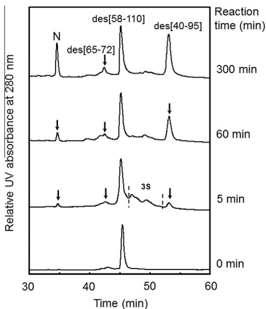
Fig. 8. HPLC chromatograms obtained by folding of isolated des[58–110] under an aerobic condition at pH 8.0 and 5 °C. The initial concentration of des[58–110] was approx. 20 \mu\text{M} .
