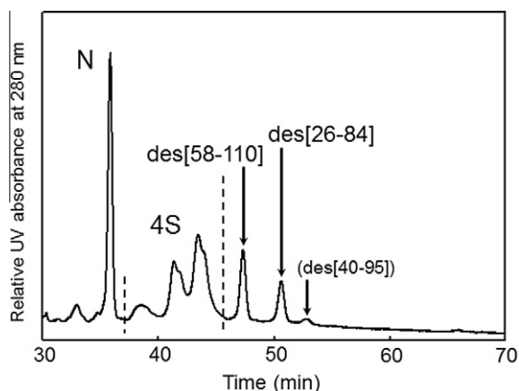
Fig. 7. An HPLC chromatogram obtained by the oxidation pulse experiment of RNase A at 15 °C and pH 8.0. Reaction conditions: [R]_0 = [DHS^{ox}]/3 = 20.7 \mu\text{M} . Oxidation pulse conditions: After 300 min of the refolding reaction, the sample solution was treated with one equivalent of DHS^{ox} at 15 °C for 3 min. See the text for details of the HPLC analysis conditions.
