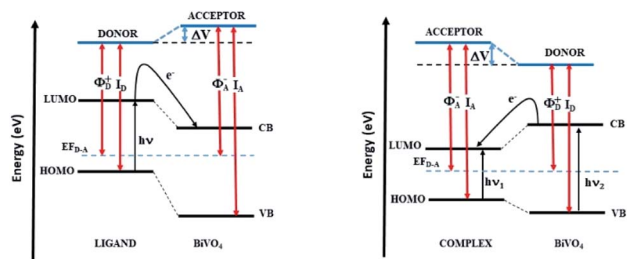
Fig. 8 Electronic band alignment at the hybrid interfaces.
