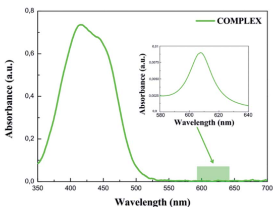
Fig. 5 Experimental UV-vis absorption spectrum measured for the COMPLEX molecule dissolved in acetonitrile/ tert -butanol (1/1).
