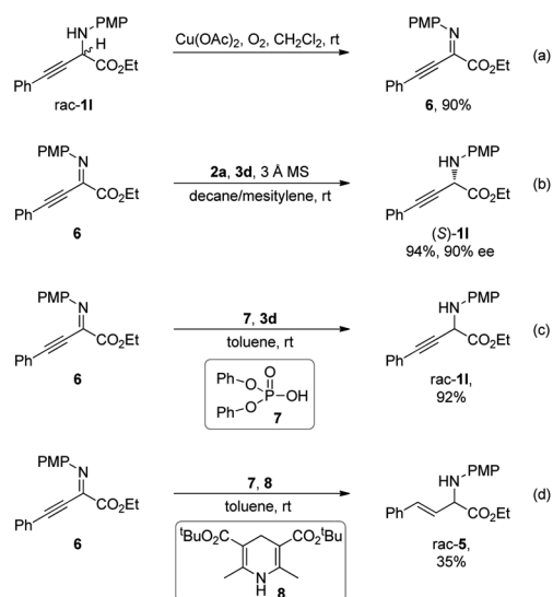
Scheme 5 Control experiments.
