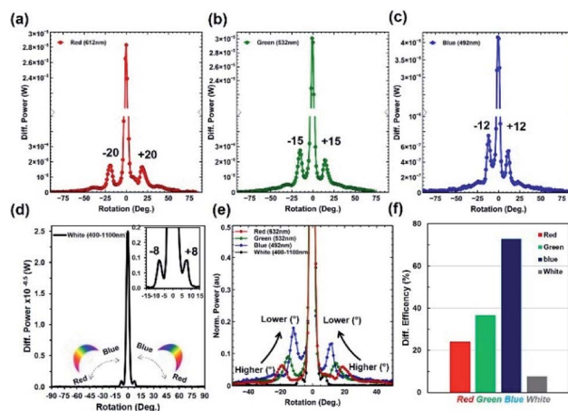
Fig. 5 Diffraction grating property of Morpho peleides -butterfly wing scales. (a–e) Diffraction power intensity as a function of rotational angle ( ^\circ ) through light illumination. (f) Diffraction efficiency with monochromatic (red, green and blue) and broadband light normal light illumination.
