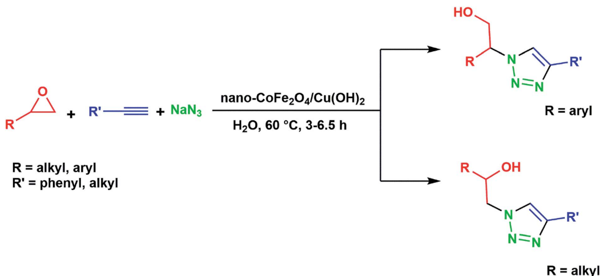
Scheme 1 One-pot synthesis of triazoles from epoxides catalyzed by \text{CoFe}_2\text{O}_4/\text{Cu}(\text{OH})_2 nanoparticles.
