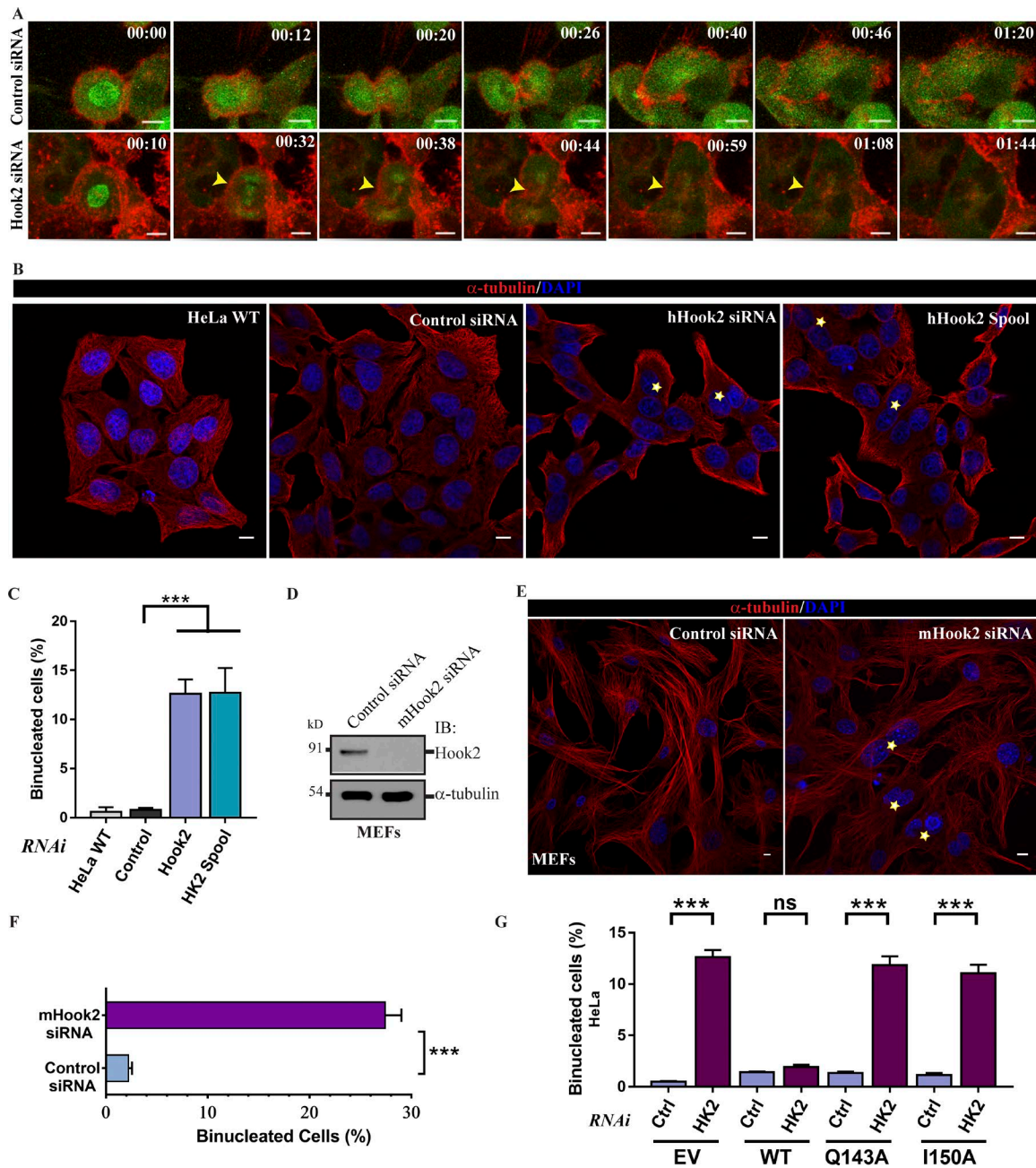
Figure 7. Hook2 depletion causes cytokinesis failure. (A) Maximum intensity projections of z-stacks of live-cell imaging of HeLa cells stably expressing GFP- \alpha -tubulin and mCherry-UtrCH and treated with control or Hook2 siRNA. Z-stack time-lapse images were acquired every 3 m for a total duration of 3 h. Bars, 10 \mu m. (B) Representative images of HeLa cells treated with indicated siRNAs. The yellow asterisks in the images indicate binucleated cells in each case. Bars, 10 \mu m. (C) Quantification of binucleated HeLa cells as described in B ( n = 5 ; 300 cells/experiment). (D) Western blot analysis confirming depletion of Hook2 in primary MEFs, and \alpha -tubulin was used as a loading control. (E) Representative images of primary MEFs treated with control or mHook2 siRNA. The yellow asterisks in the images indicate binucleated cells in each case. Bars, 10 \mu m. (F) Quantification of binucleated primary MEFs as described in E ( n = 5 ; 300 cells/experiment). (G) Quantification of the percentage of binucleated cells in siRNA-resistant Hook2 (WT/Q143A/I150A) transfected HeLa cells treated with control or Hook2 siRNA ( n = 3 ; 200 cells/experiment). Data represent mean \pm SD (ns, not significant; ***, P < 0.001 ; Student's t test).
