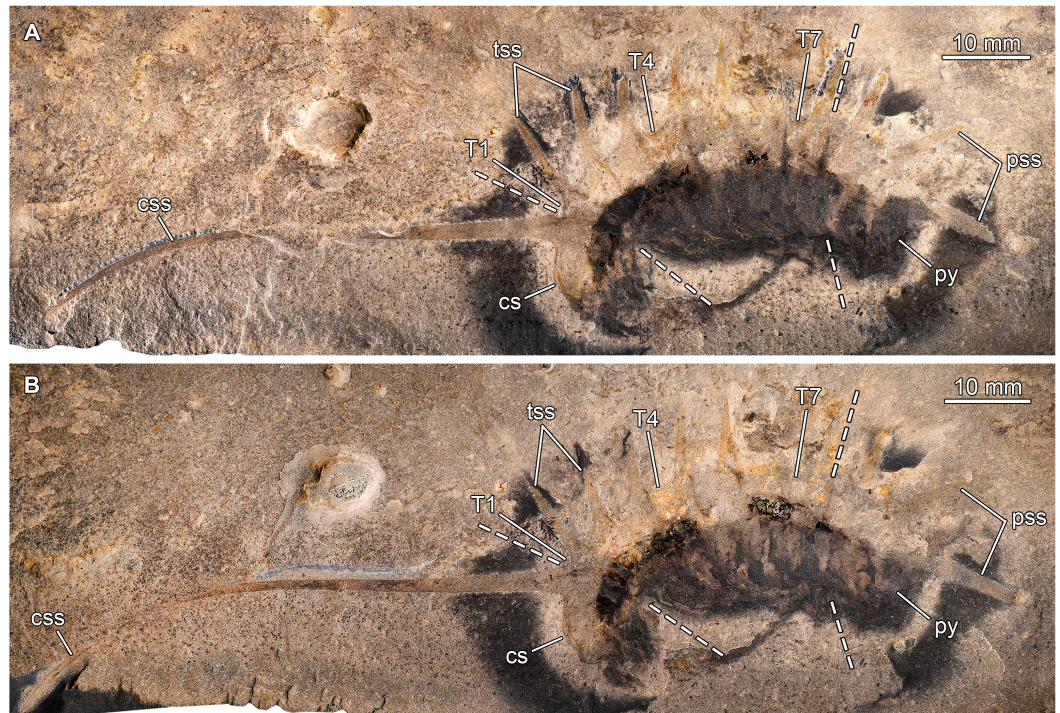
Figure 5 Thelxiope spinosa (Conway Morris & Robison, 1988) from the Cambrian (Drumian) Wheeler Formation in the House Range of Utah, USA. (A, B) General views of holotype specimen USNM424114 (immersed in dilute ethanol; cross polarized light; photo credit: Sarah Losso). (A) Part. (B) Counterpart (mirrored). Abbreviations: cs , cephalic shield; css , cephalic sagittal spine; pss , pygidial sagittal spines; py , pygidium; T , thoracic tergite; tss , thoracic sagittal spines.
