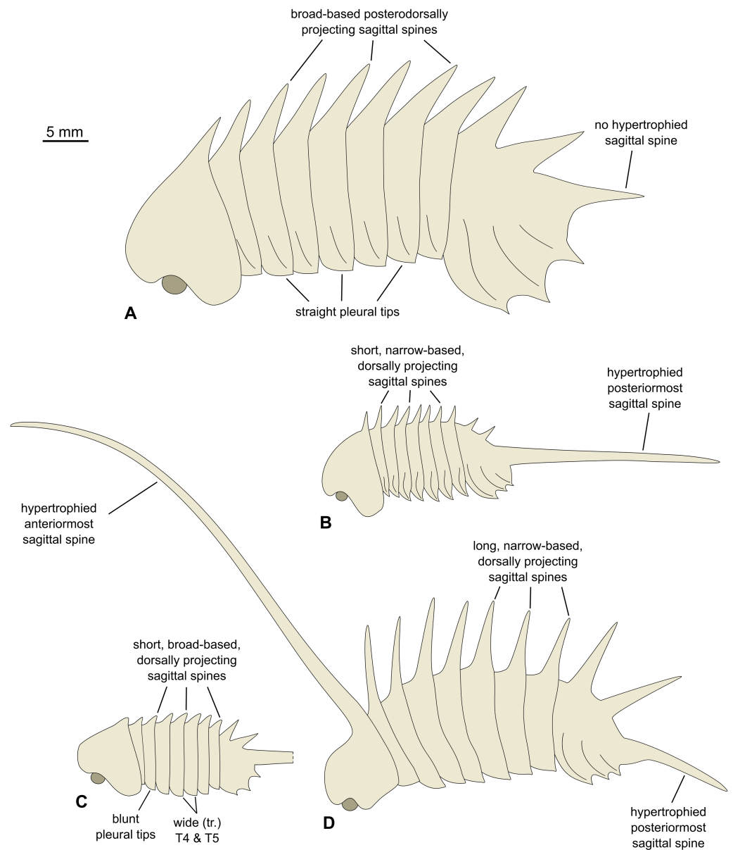
Figure 8 Morphological reconstructions of the four species of Thelxiope and their diagnostic features. (A) Thelxiope holmani sp. nov., Drumian Wheeler Shale. (B) Thelxiope palaeoethalassia (type species), Wuliuan Burgess Shale. (C) Thelxiope sp. nov. A, Tremadocian, lower Fezouata Shale. (D) Thelxiope spinosa , Drumian Wheeler Shale. Note that the morphology of the lateral margins of the dorsal exoskeleton in T. spinosa , and the presence of marginal and some sagittal spines on the cephalic shield and pygidium of Thelxiope sp. nov. A have been extrapolated from congeneric species. Credit for all drawings: Javier Ortega-Hernández.
