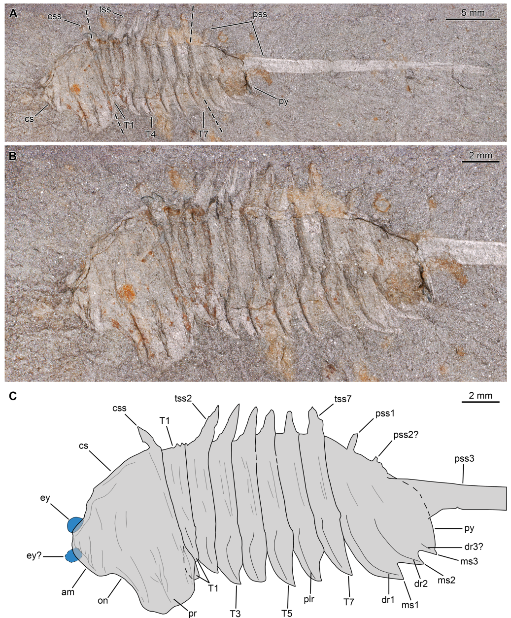
Figure 2 Thelxiopae palaeothalassia Simonetta & Delle Cave, 1975 from the Cambrian (Wuliuan) Burgess Shale Formation, British Columbia, Canada. (A, B) Holotype specimen USNM144914 (immersed in dilute ethanol, cross polarized light), general (A) and detailed (B) views. (C) Interpretative drawing (credit: Rudy Lerosey-Aubril). Abbreviations: am , anterior margin of cephalic shield; cs , cephalic shield; css , cephalic sagittal spine; dr , dorsal ridge; ey , eye; ms , marginal spine; on , optical notch; plr , tergopleural ridge; pr , tergopleural region; pss , pygidial sagittal spine; py , pygidium; T , thoracic tergite; tss , thoracic sagittal spine.
