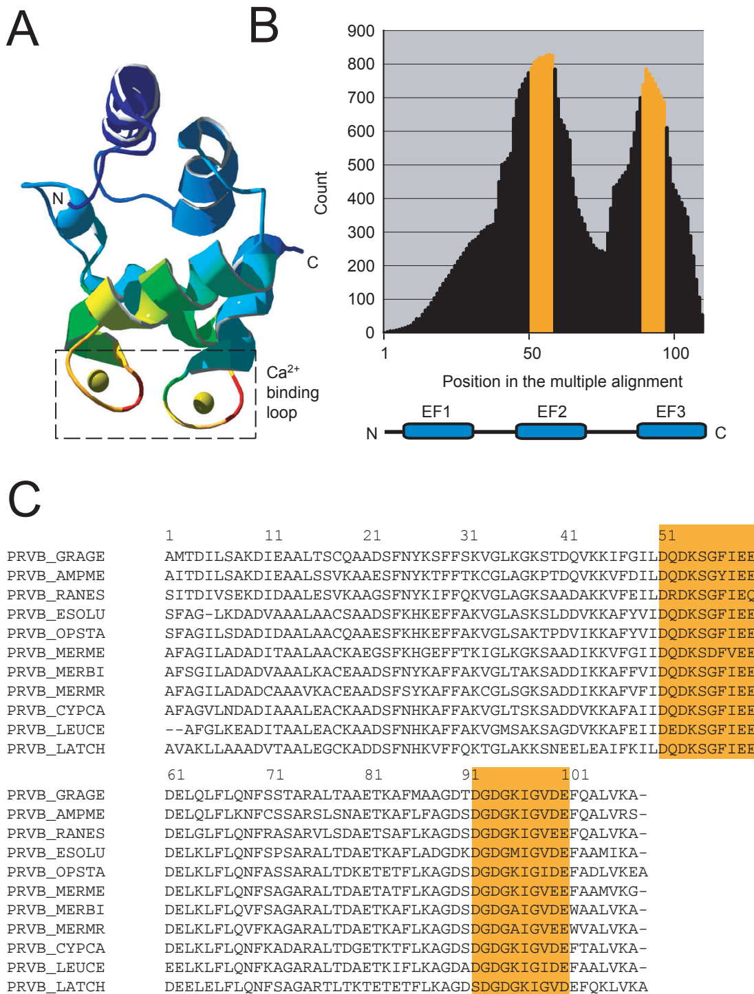
Figure 7 Mapping the HMM histogram to the crystal structure of parvalbumin B. A) The HMM histogram mapped onto the crystal structure (PDB code: 1CDP) of parvalbumin B. Using the same conventions as Fig. 5A, the Ca 2+ binding loops of two EF-hand motifs have a high occurrence level. B) The HMM histogram of the parvalbumin B subfamily with an e-value cutoff of 0.1. The orange regions in the histogram reflect the segments encoding the Ca 2+ binding loops. Below the histogram is the domain layout. The blue rectangle represents the EF-hand motif (EF). C) The MSA of the parvalbumin B subfamily. Using the same conventions as Fig. 5C, the Ca 2+ binding loops are highlighted orange.
