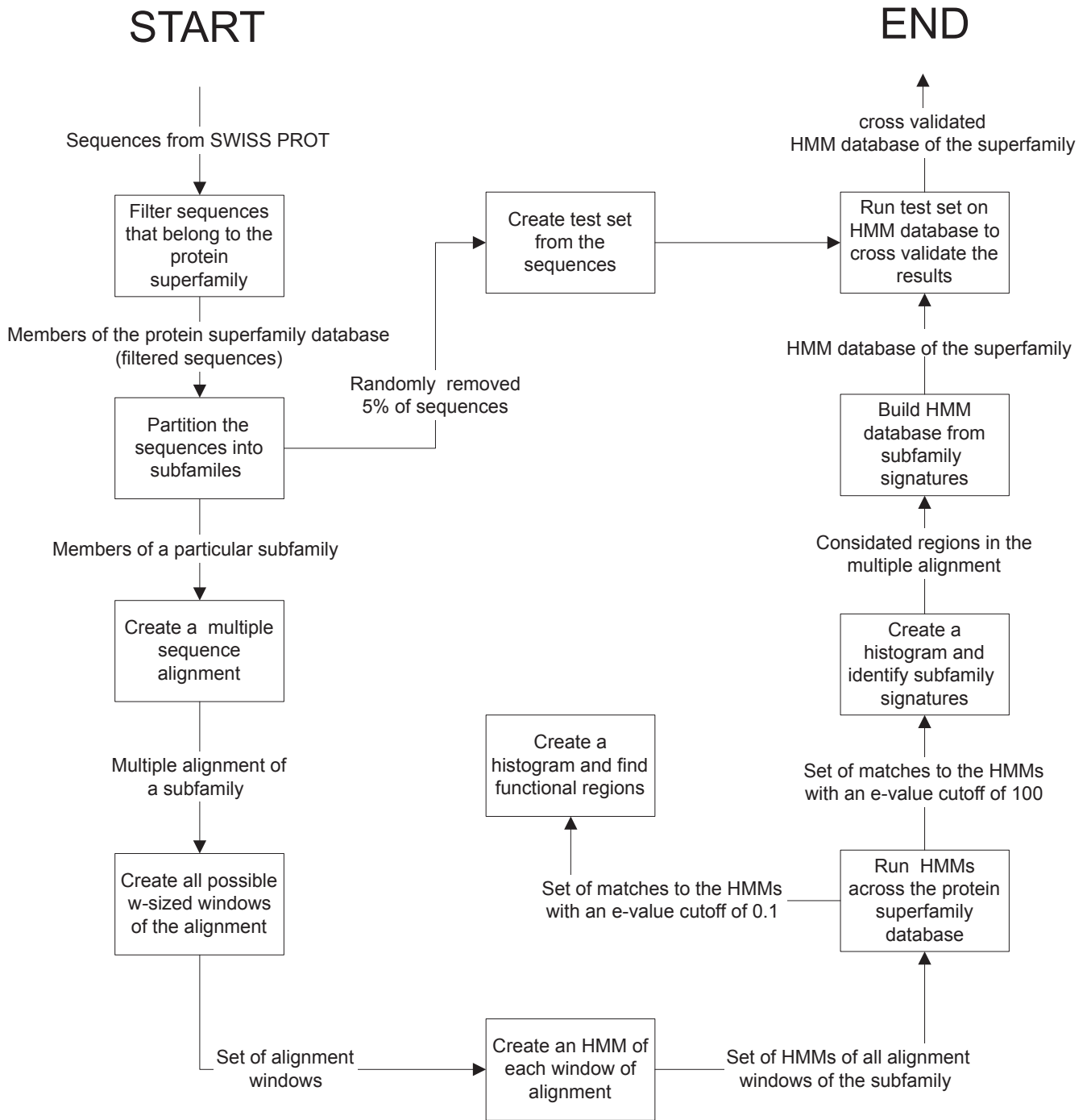
Figure 1 Flow diagram of the method. First, filter a primary database using a profile or motif database for a subset of sequences that will comprise the protein superfamily database. Then, partition the protein superfamily database into subfamilies depending on the criterion for a subfamily. Then, build an MSA for each subfamily and build HMMs of all w width windows of the MSA. Finally, tabulate matches with an e-value under 100 to identify subfamily signatures for the HMM database of the superfamily and tabulate matches with e-value under 0.1 to identify potentially significant functional regions in the subfamily.
