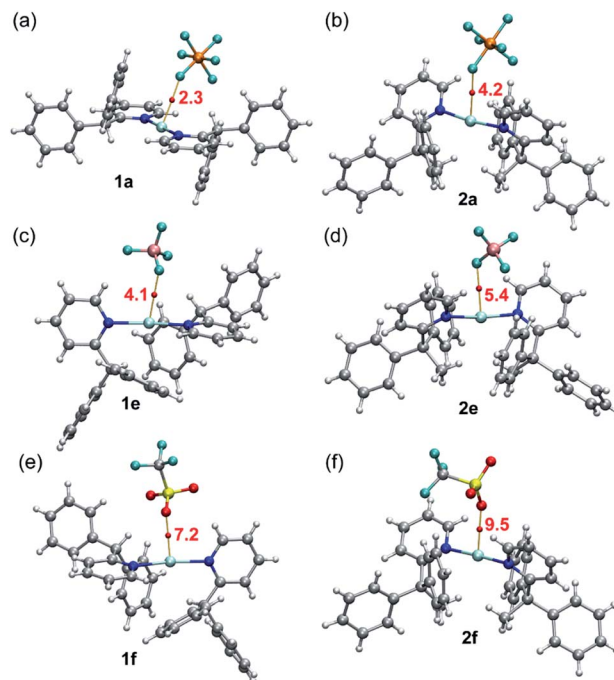
Fig. 8 QTAIM analysis (only the Ag⋯anion contact is represented for clarity) of compounds 1a (a), 2a (b), 1e (c), 2e (d), 1f (e) and 2f (f). The dissociation energies are indicated in red adjacent to the bond CPs (red spheres).
