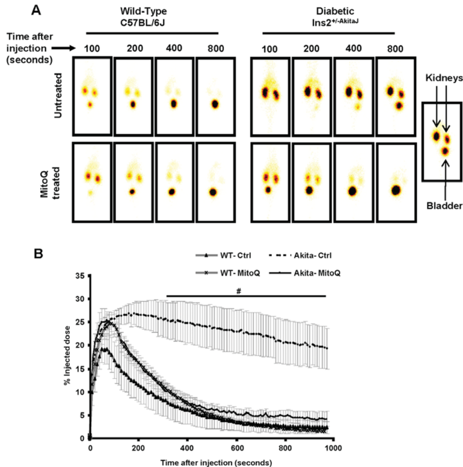
Figure 1 MitoQ treatment prevents renal tubular dysfunction in Ins2^{+/-AkitaJ} mice as determined by ^{99m}Tc -MAG3 clearance
