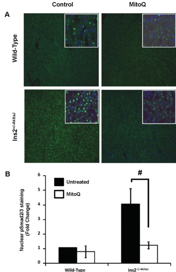
Figure 8 MitoQ treatment inhibits phospho-Smad2/3-mediated signalling in the diabetic kidney
