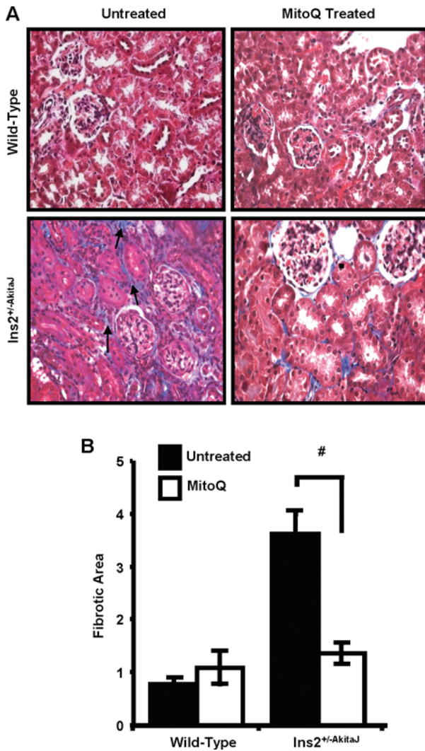
Figure 7 MitoQ treatment decreases diabetes-induced renal interstitial fibrosis
