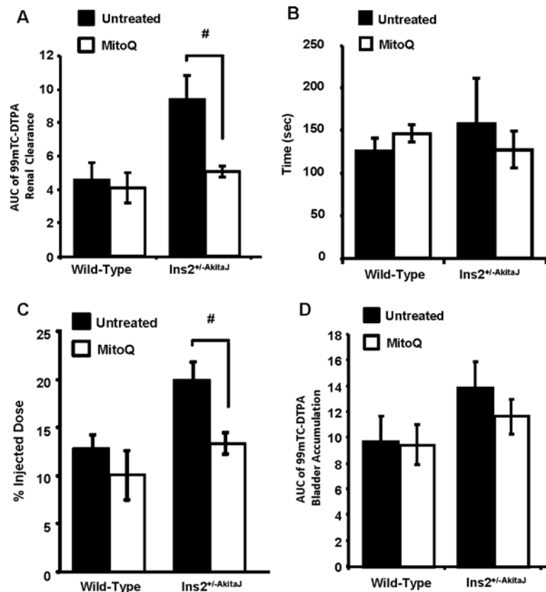
Figure 4 Preservation of glomerular function by MitoQ in Ins2^{+/-AkitaJ} mice
