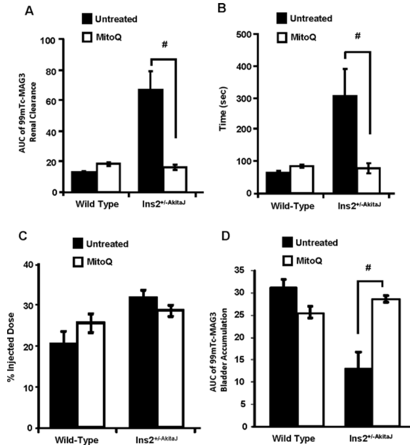
Figure 2 Protection of renal tubular function by MitoQ in Ins2^{+/-AkitaJ} mice
