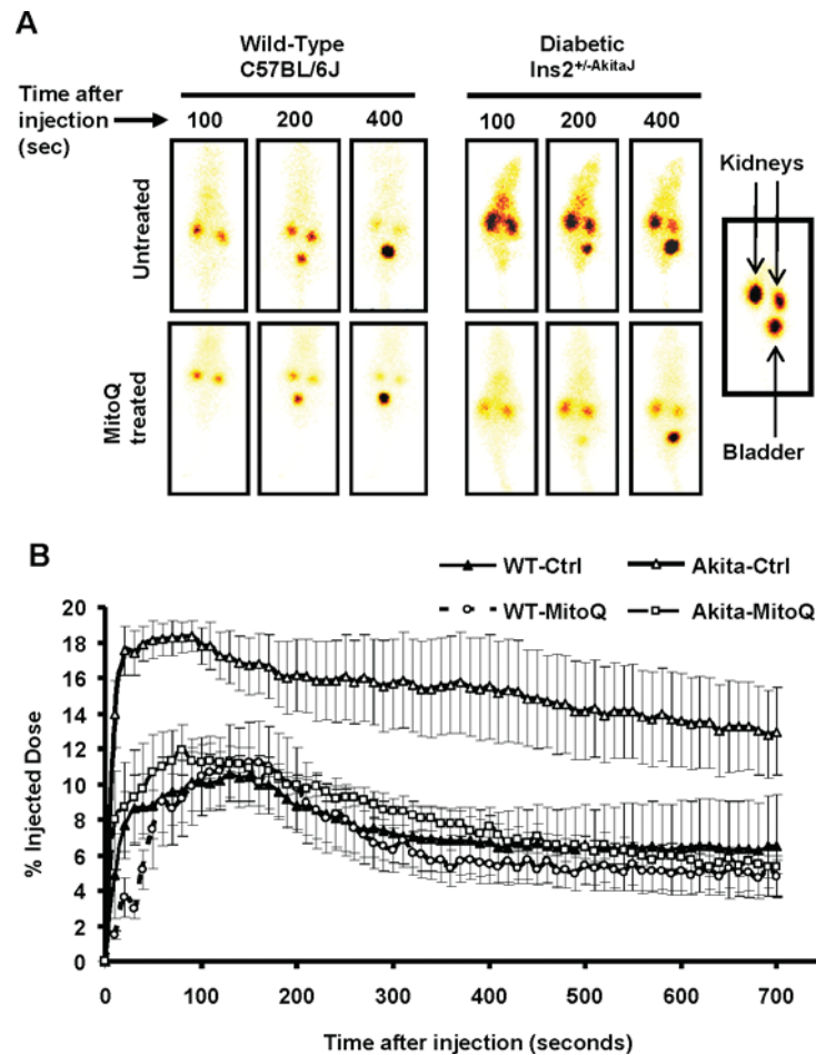
Figure 3 MitoQ protects against diabetic glomerular dysfunction in Ins2^{+/-AkitaJ} mice as determined by the ^{99m}Tc -DTPA clearance
