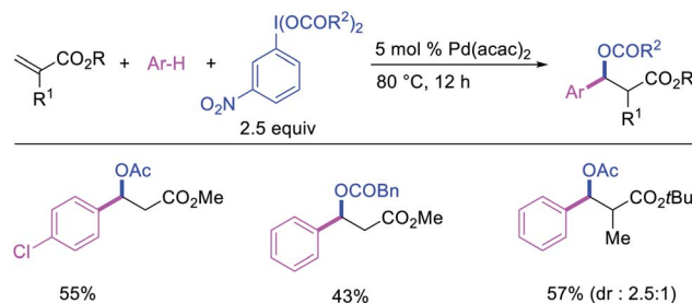
Scheme 22 Pd-catalyzed 1,1-aryloxygenation via C–H activation.
