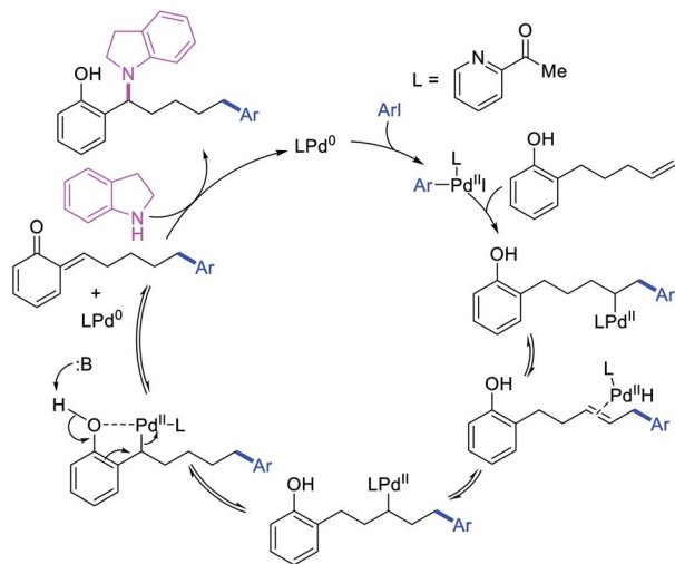
Scheme 66 Mechanism of the Pd-catalyzed 1, n -aryliodoloylation.
