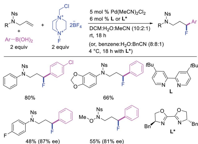
Scheme 26 Pd-catalyzed 1,1-aryloxygenation.
