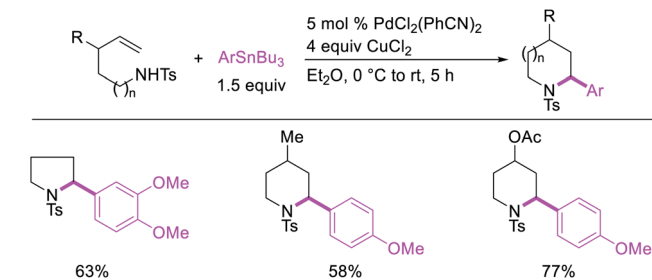
Scheme 18 Pd-catalyzed 1,1-arylamination.
