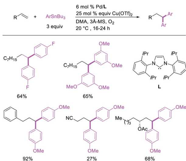
Scheme 8 Pd-catalyzed 1,1-homodiarylation with arylin reagents.
