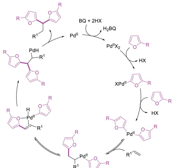
Scheme 7 Mechanism of the Pd-catalyzed 1,1-difurylation.
