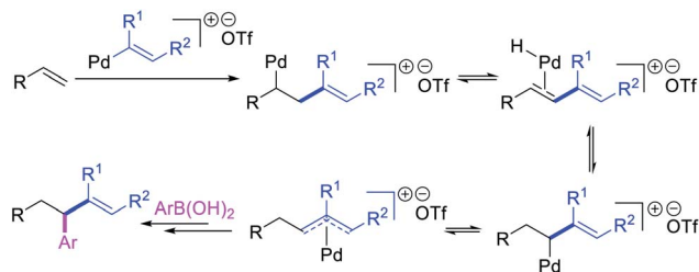
Scheme 12 Mechanism of the Pd-catalyzed 1,1-arylvinylation.
