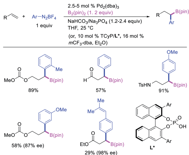
Scheme 29 Pd/CAPT-catalyzed 1,1-arylborylation.
