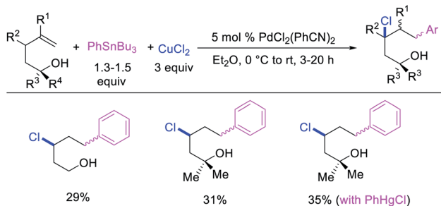
Scheme 56 Pd-catalyzed 1,3-arychlorination.
