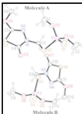
Fig. 1. The molecular structure of the title compound with the atom numbering scheme. Displacement ellipsoids are drawn at the 50% probability level. H atoms are presented as a small spheres of arbitrary radius.
